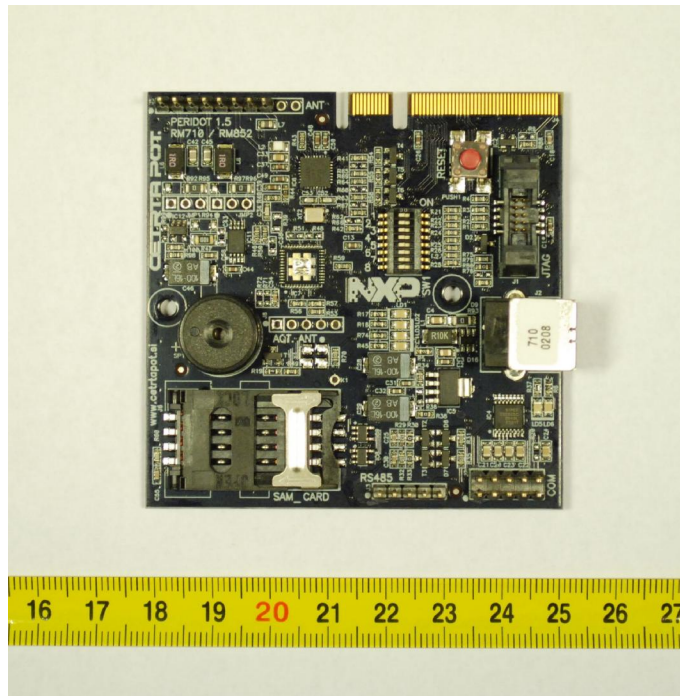
Picture 1: RD710 reader pcb - top side
