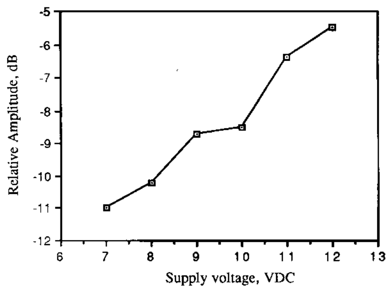
Figure 6.4. Relative emission at 310.0 MHz vs. supply voltage. (pulsed emission)
