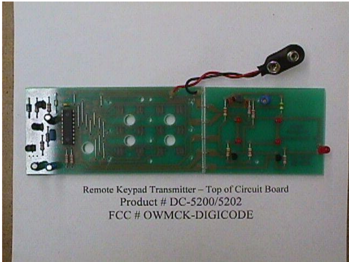
DigiCode 5200/5202 Transmitter PCB (top)
