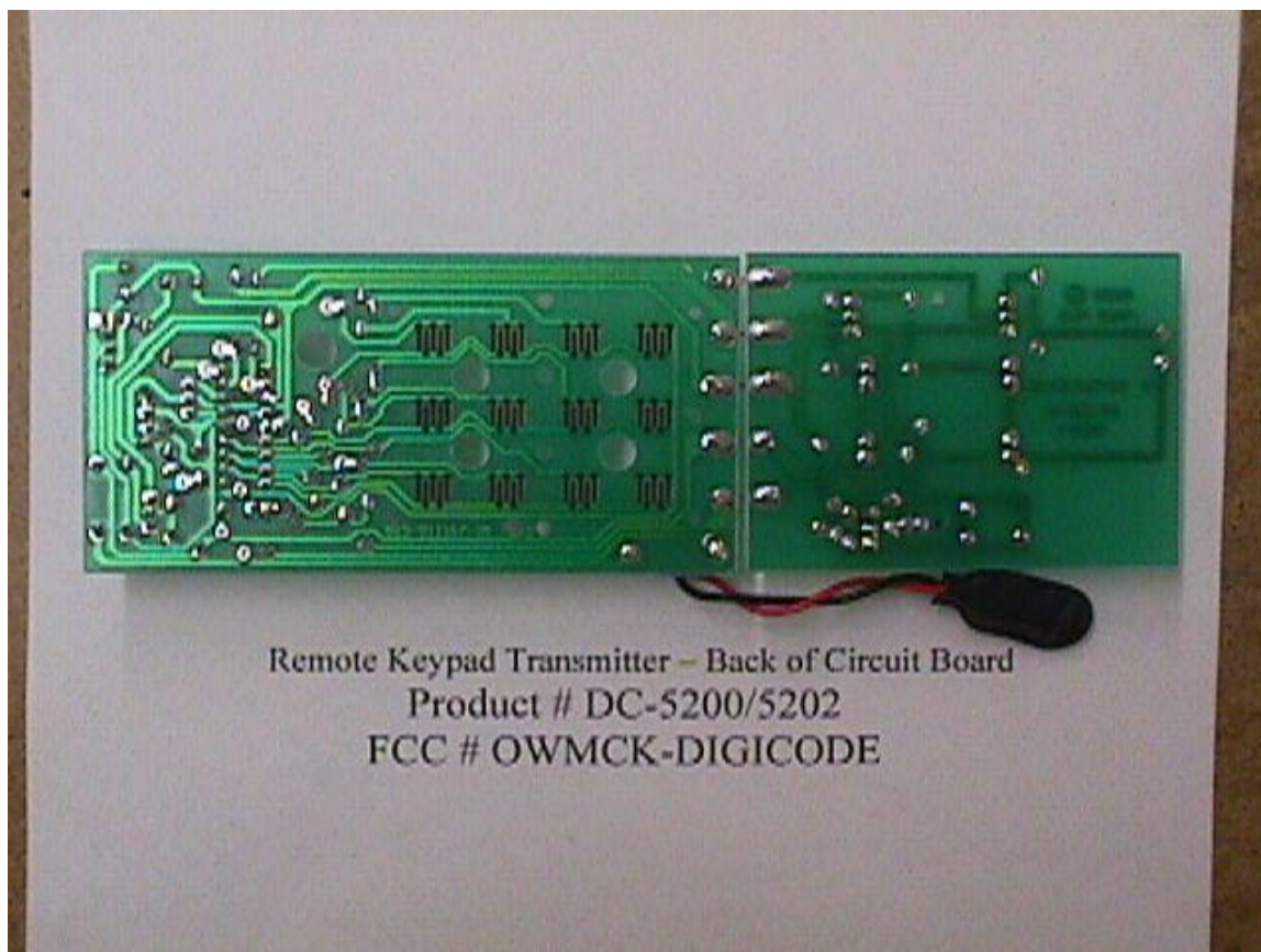
DigiCode 5200/5202 Transmitter PCB (bottom)
