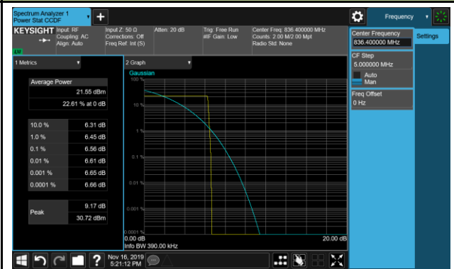
Channel 189 (836.4MHz)
