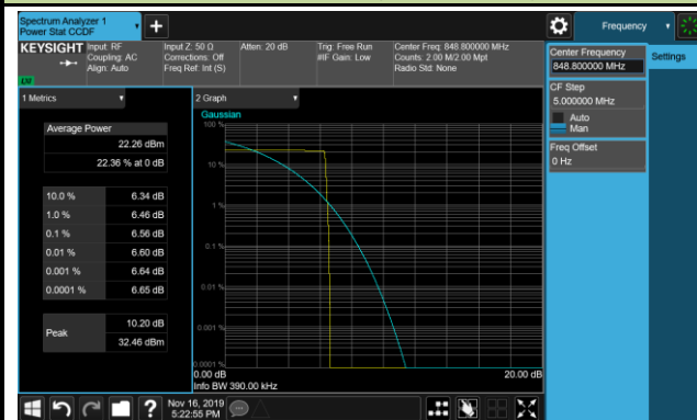
Channel 251 (848.8MHz)
