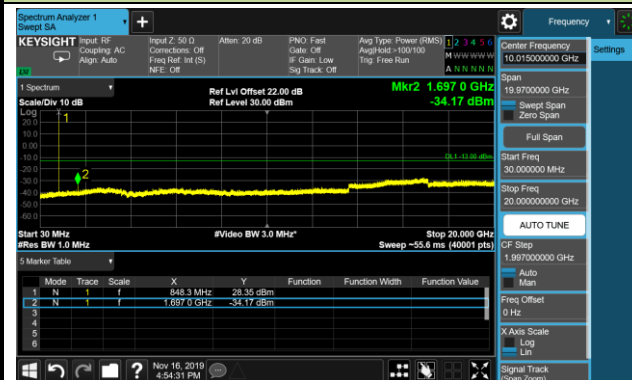
Channel 251 (848.80MHz)
