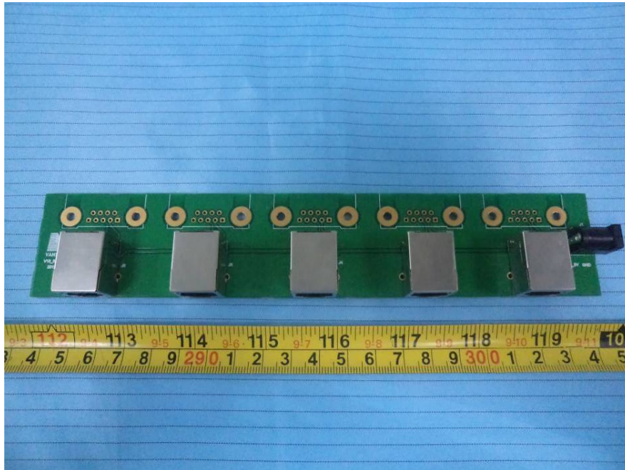
V10-8-POWER Board Top View
