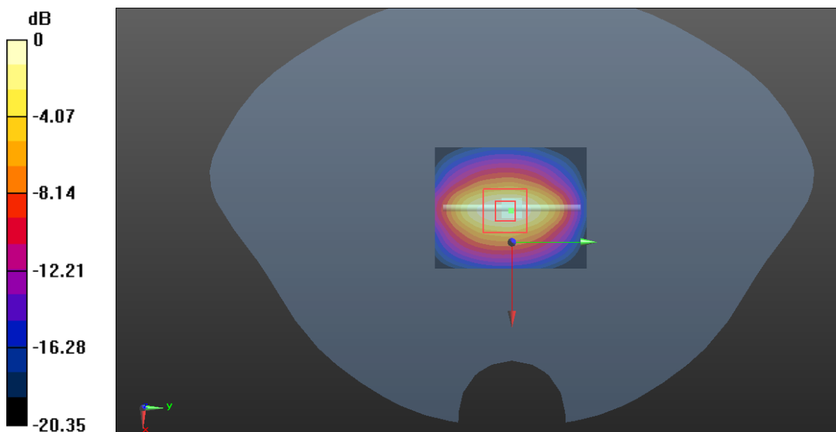
0 dB = 6.44 W/kg = 8.09 dBW/kg
