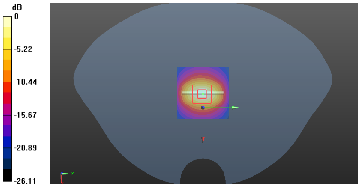
0 dB = 9.45 W/kg = 9.75 dBW/kg
