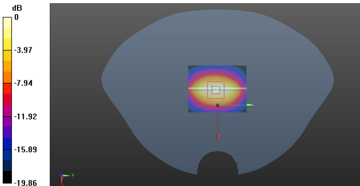
0 dB = 5.59 W/kg = 7.47 dBW/kg
