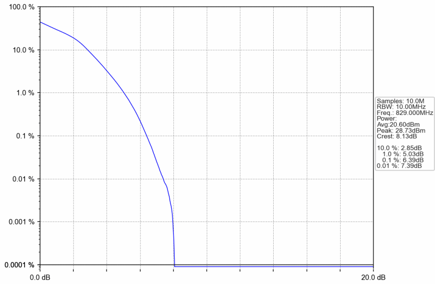
Band5_10MHz_16QAM_LCH_829MHz_RB_50_0_NTNV
