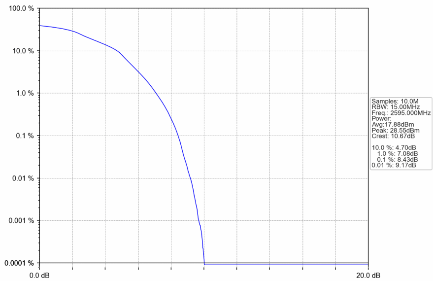
Band38_15MHz_16QAM_MCH_2595.000MHz_RB_75_0_NTNV
