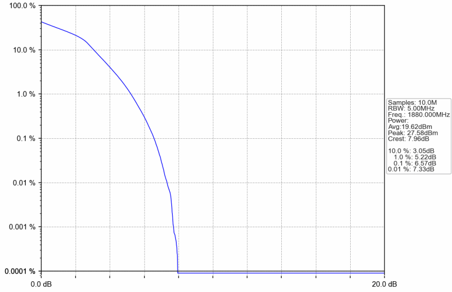
Band2_3MHz_16QAM_MCH_1880MHz_RB_15_0_NTNV
