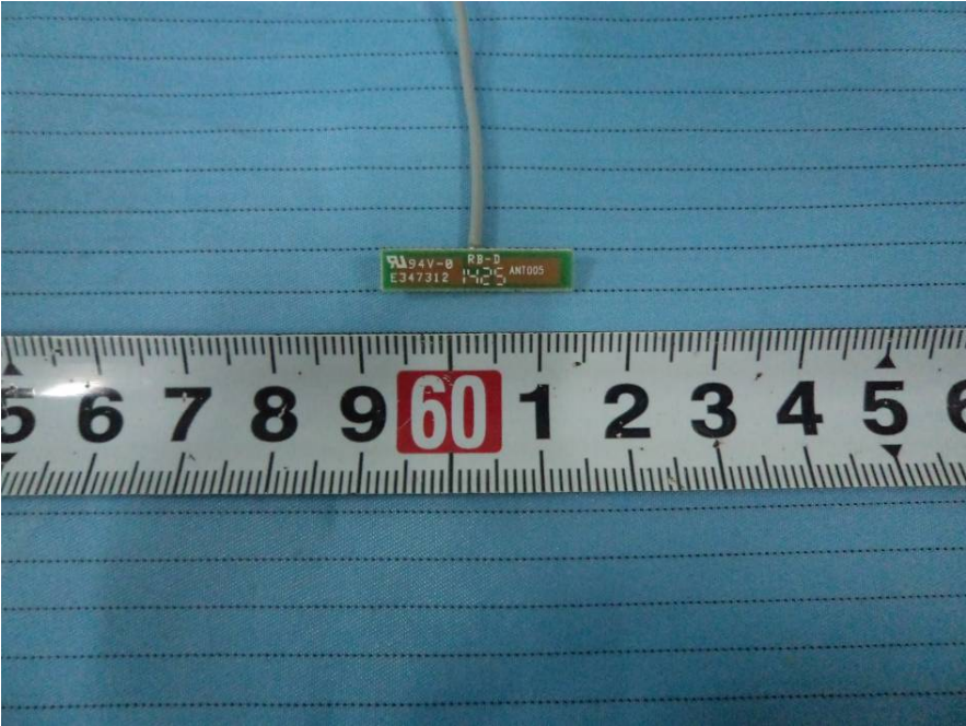
EUT – Antenna 1 Front View
