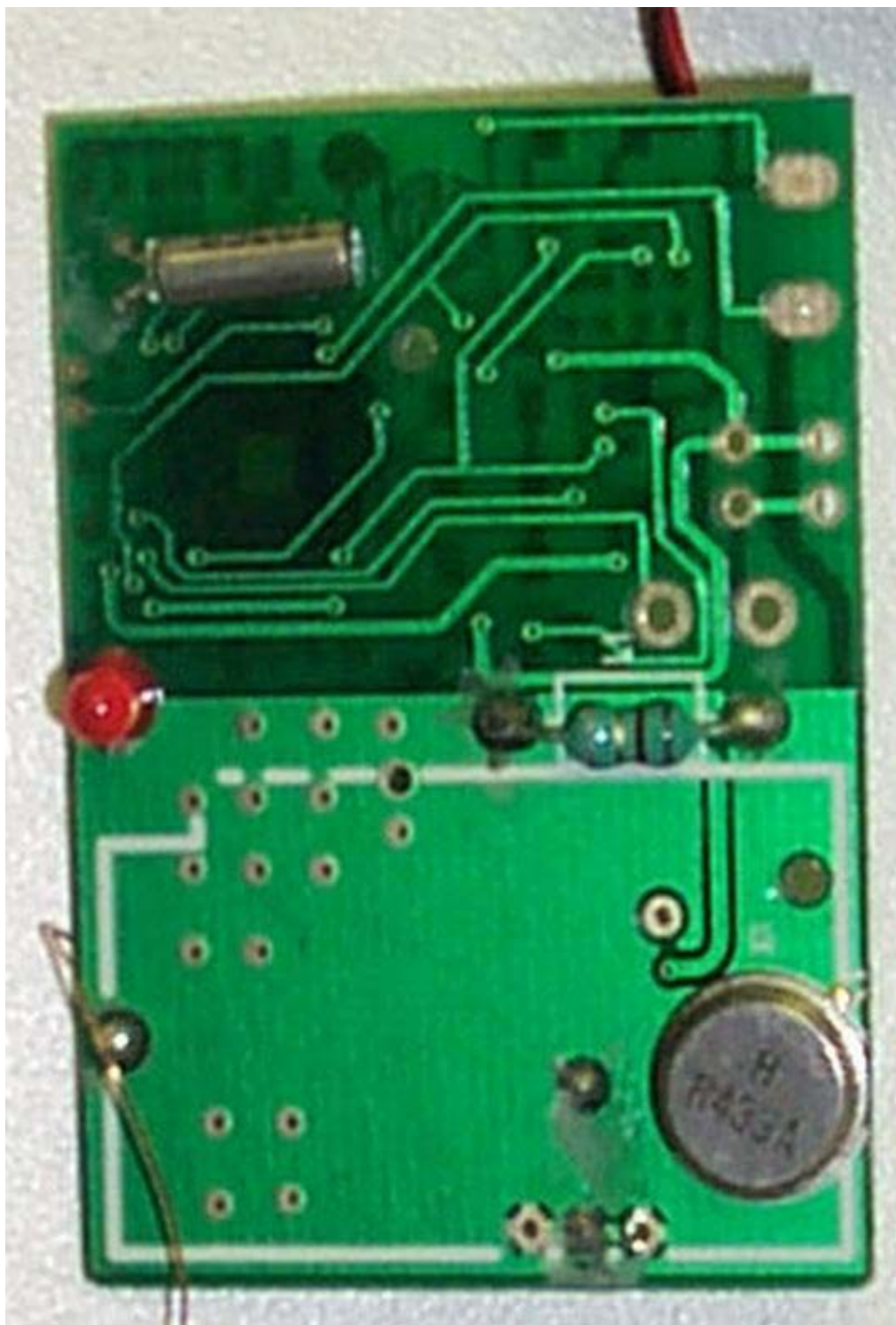
Figure 6.5 Foil Side
