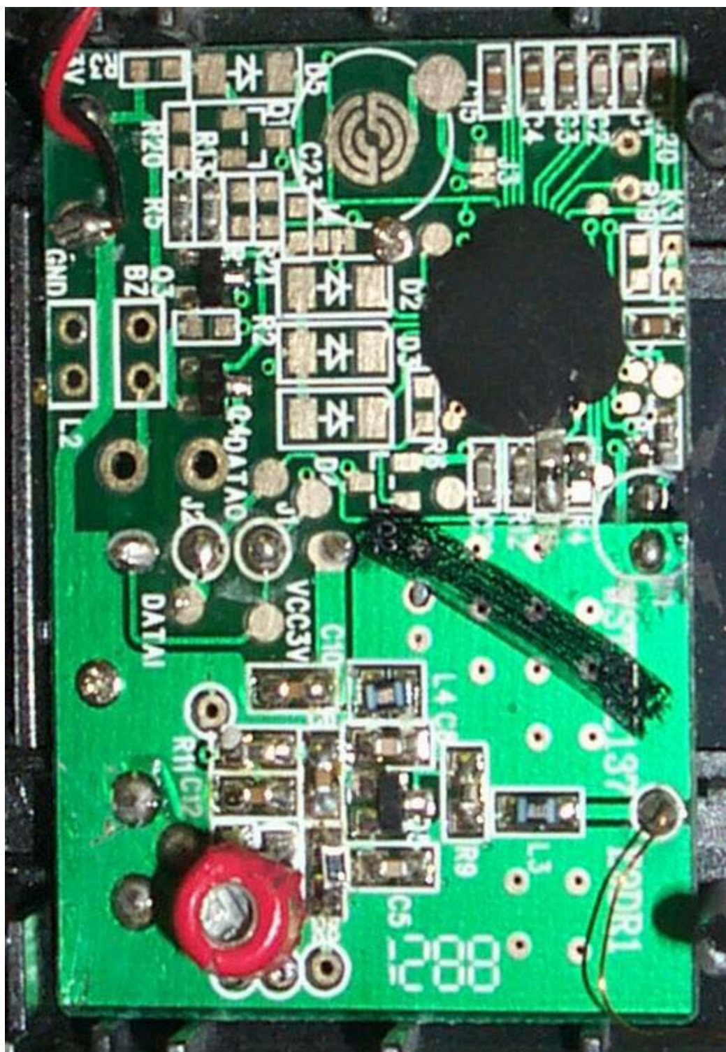
Figure 6.4 Component Side
