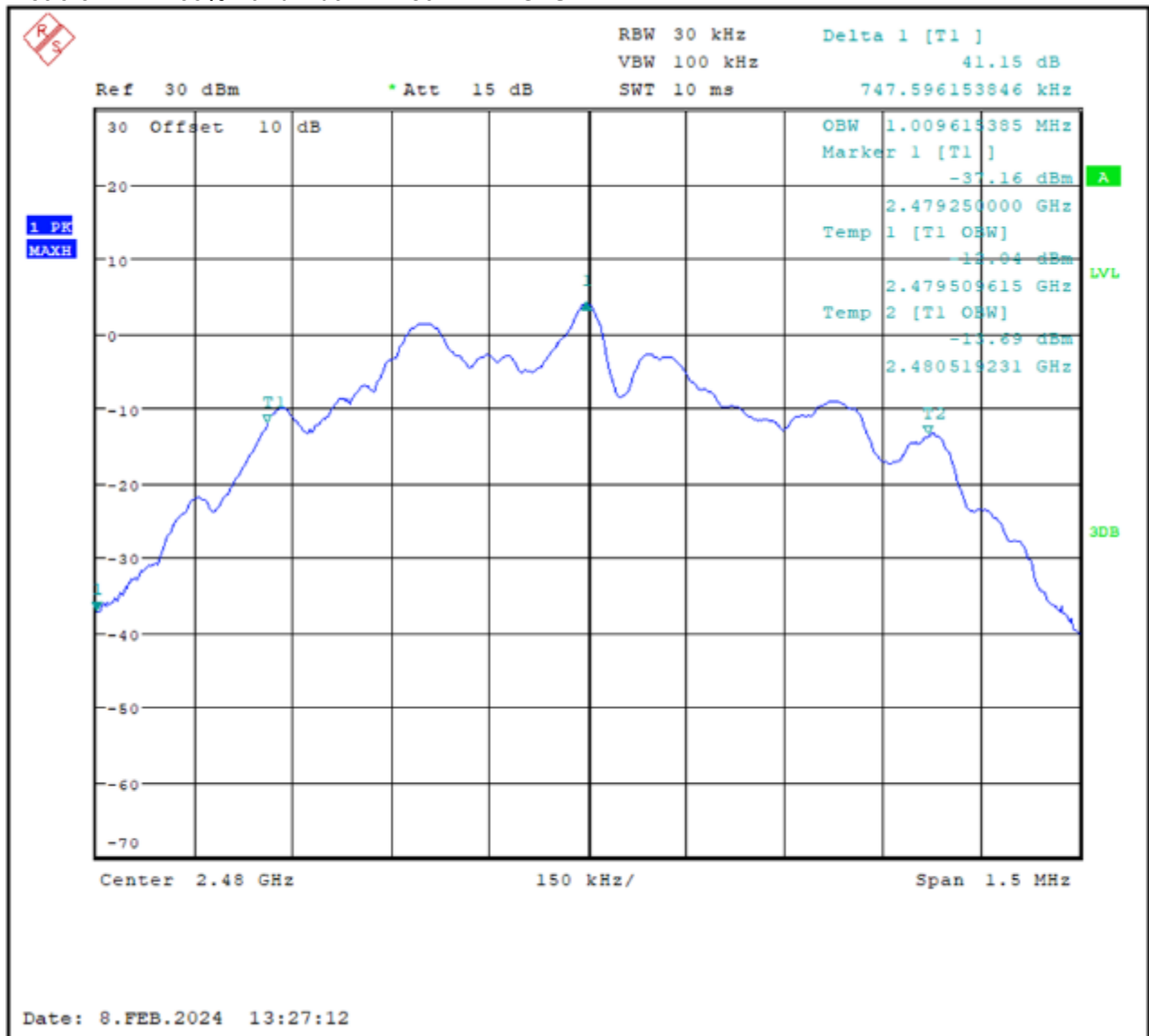
Plot 6-3: 99% Bandwidth – 2480 MHz – GFSK
