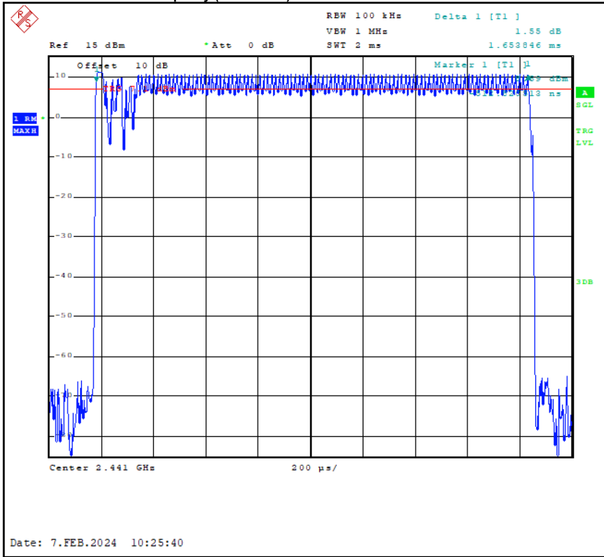
Plot 9-1: Time of Occupancy (Dwell Time)
