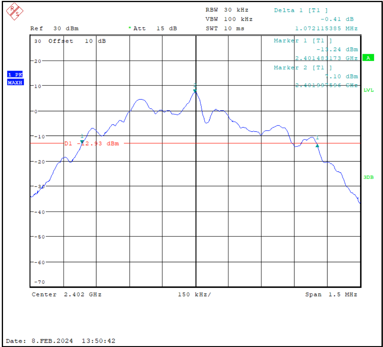
Plot 6-1: 20 dB Bandwidth – 2402 MHz – GFSK
