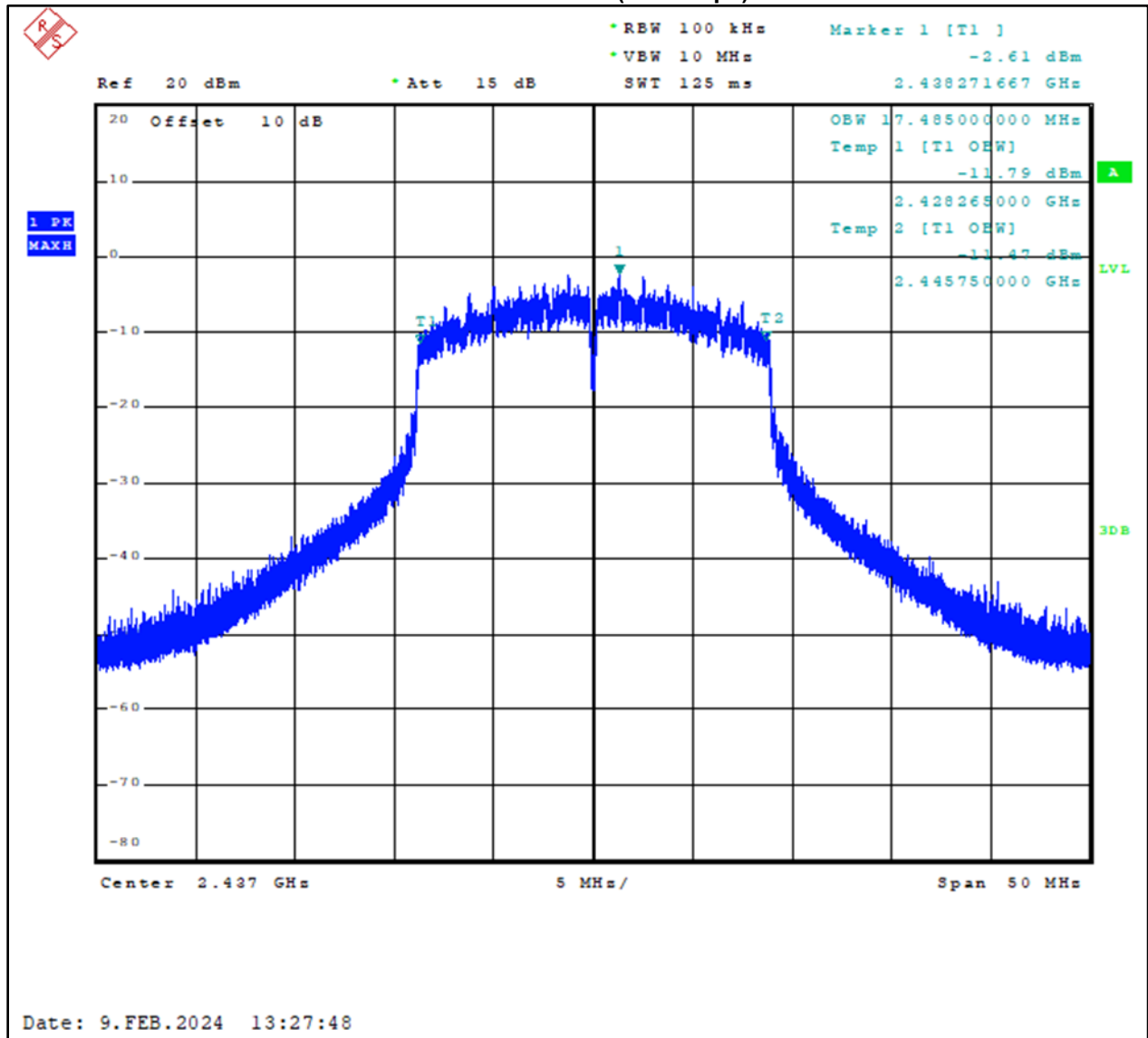
Plot 6-5: 99% Bandwidth – 2437 MHz – 802.11b (11.0 Mbps)
