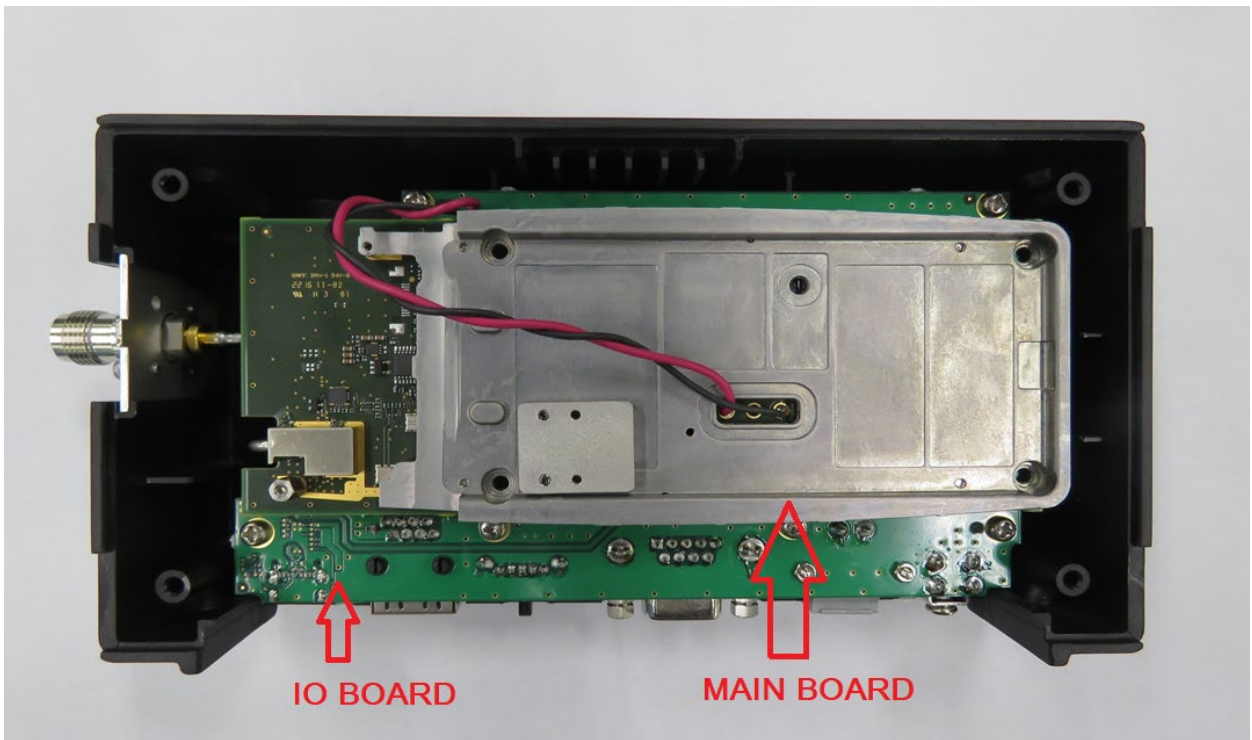
Internal Assembly
