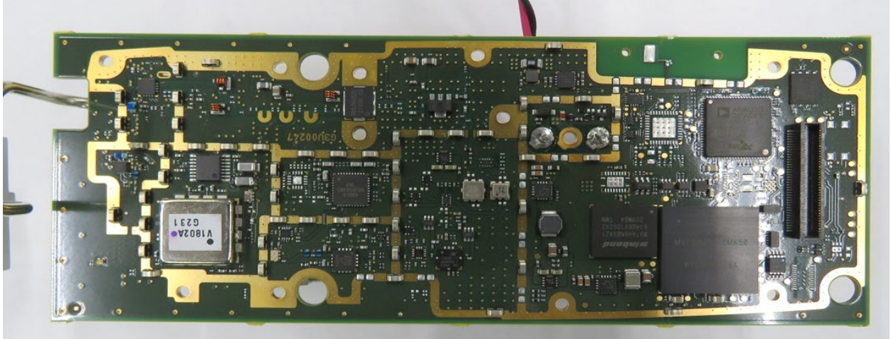
Main Board Bottom Side with Shield Removed
