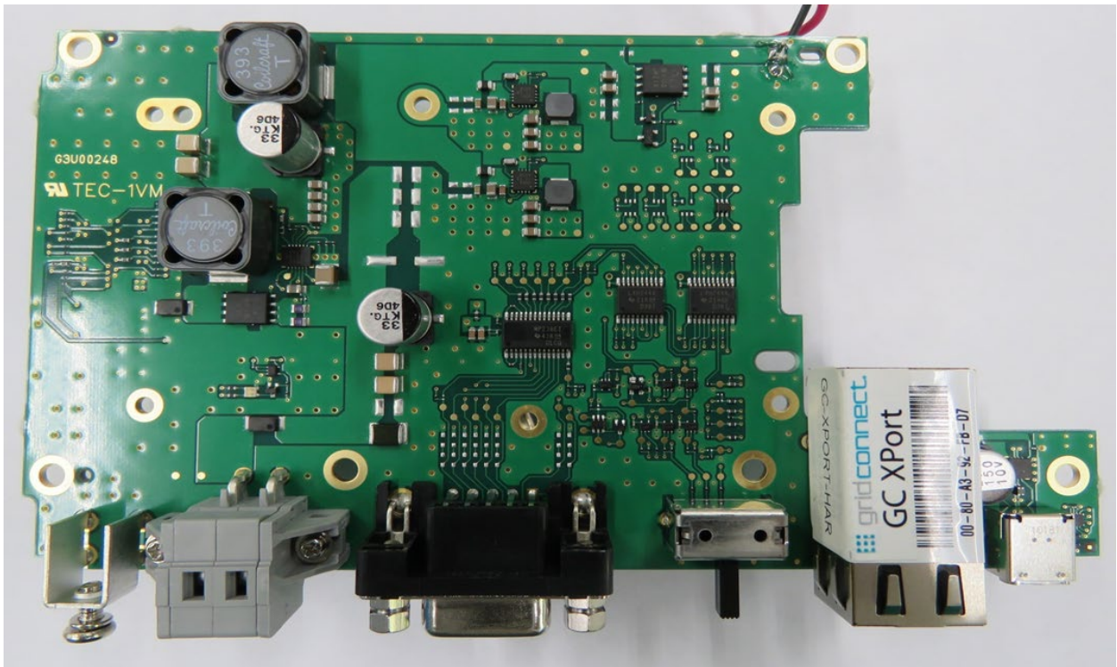
IO Board Top Side
