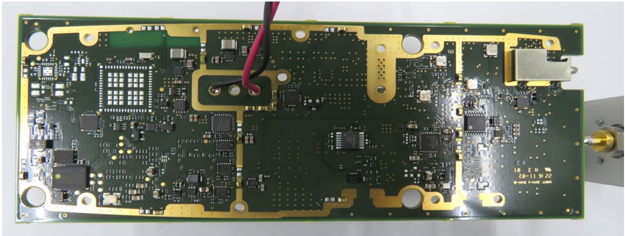
Main Board Top Side with Shield Removed
