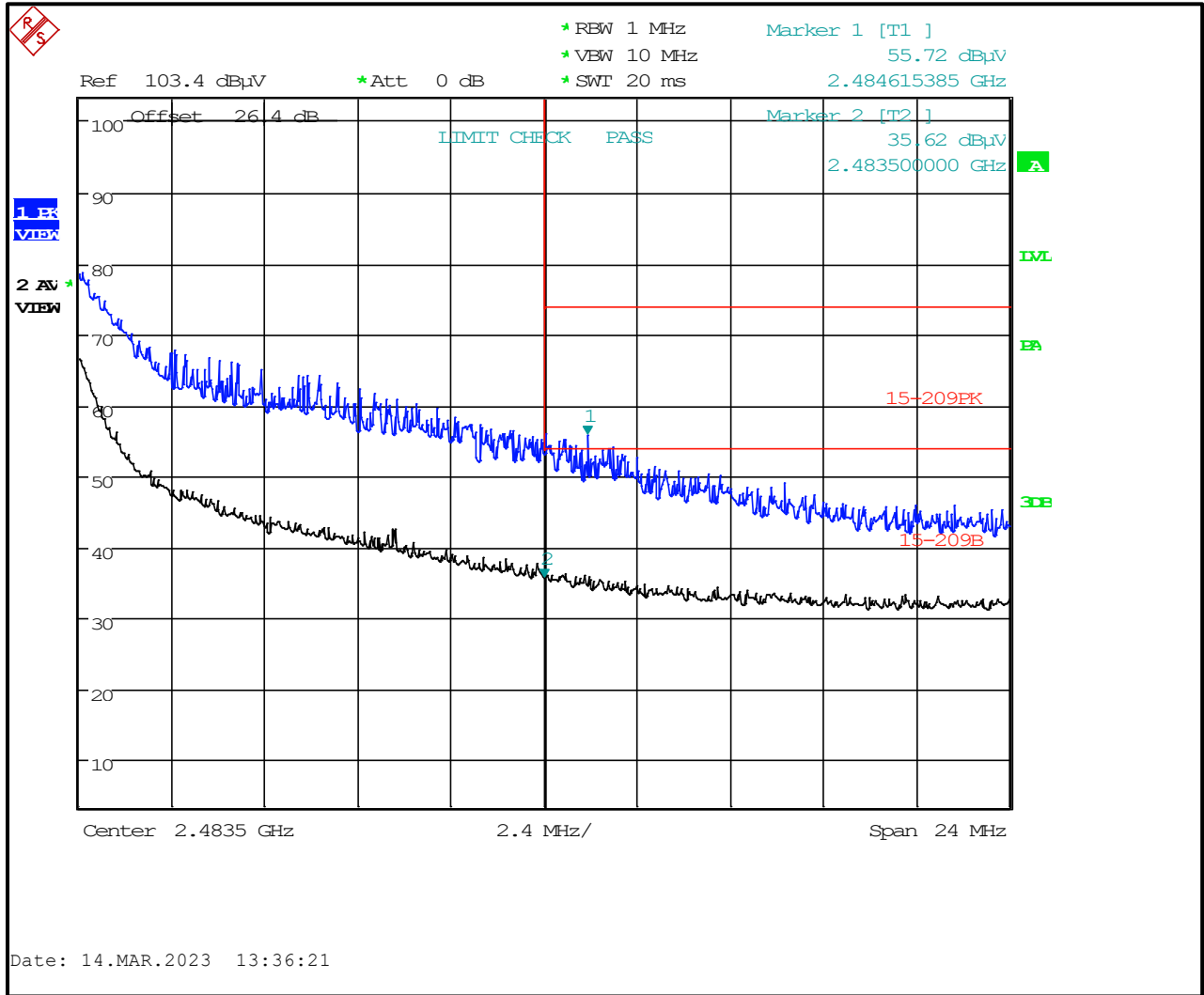
Plot 4-6: Upper Band Edge – 802.11n (65.0 Mbps)
