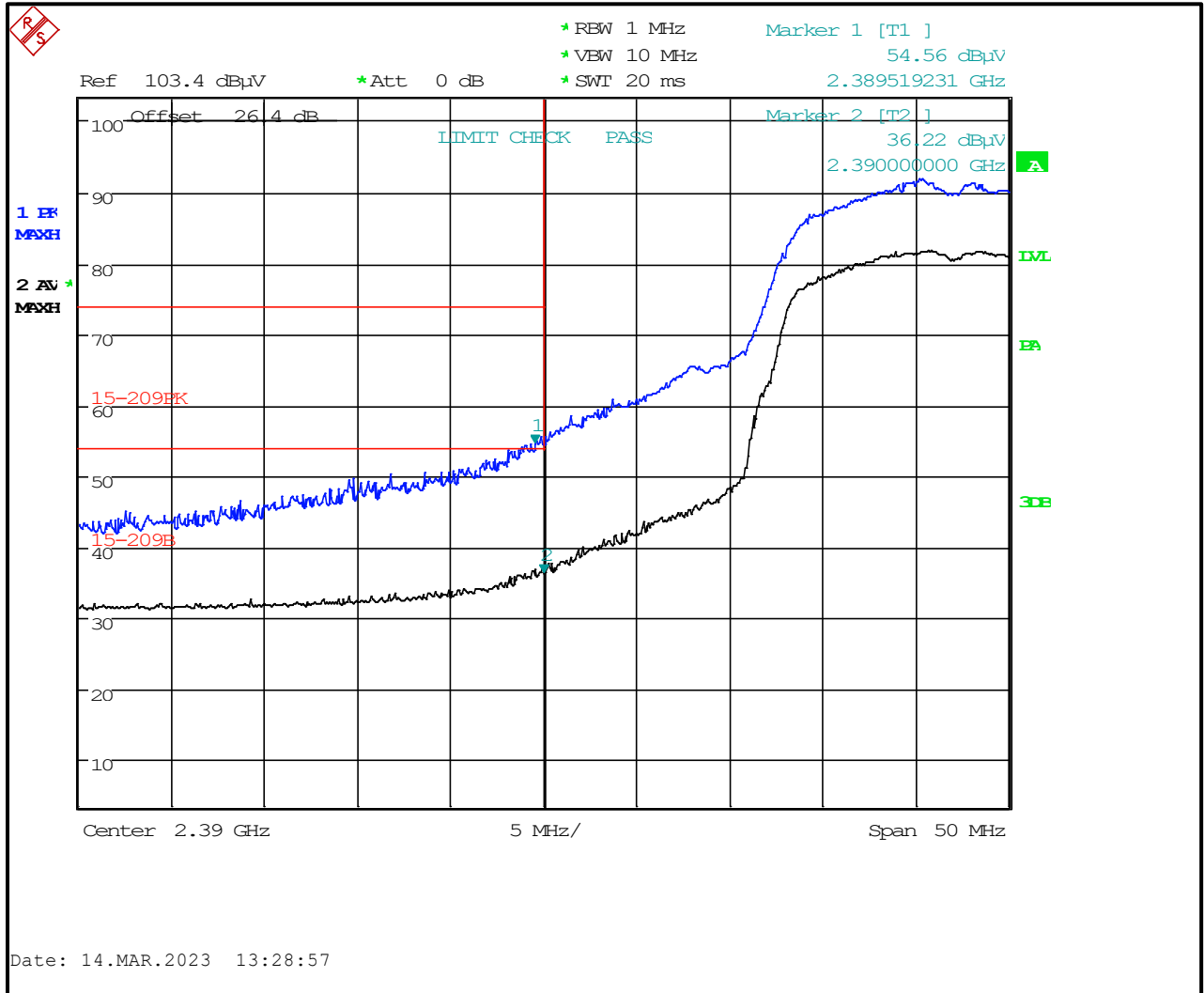
Plot 4-5: Lower Band Edge – 802.11n (65 Mbps)
