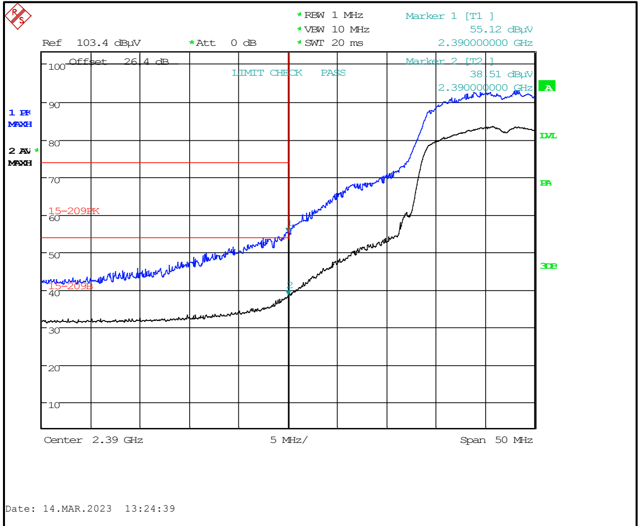
Plot 4-3: Lower Band Edge – 802.11g (12.0 Mbps)
