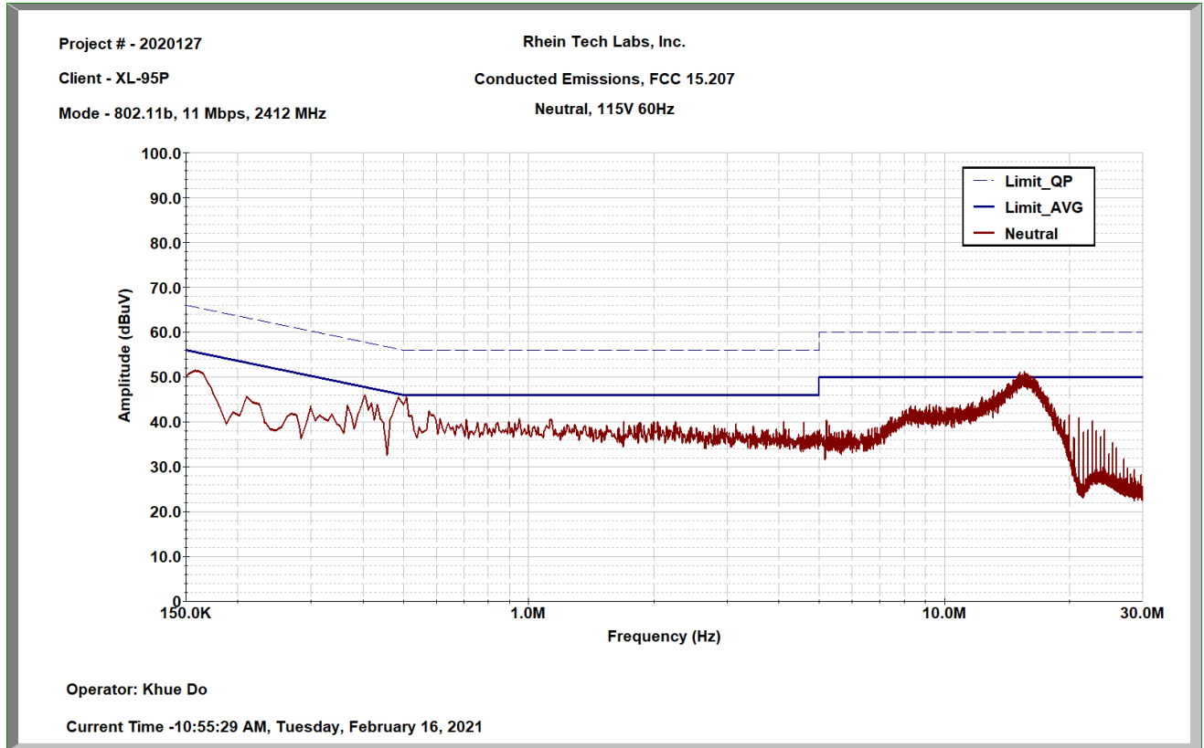
Plot 8-1: Conducted Emissions, AC, Neutral, 2412 MHz
