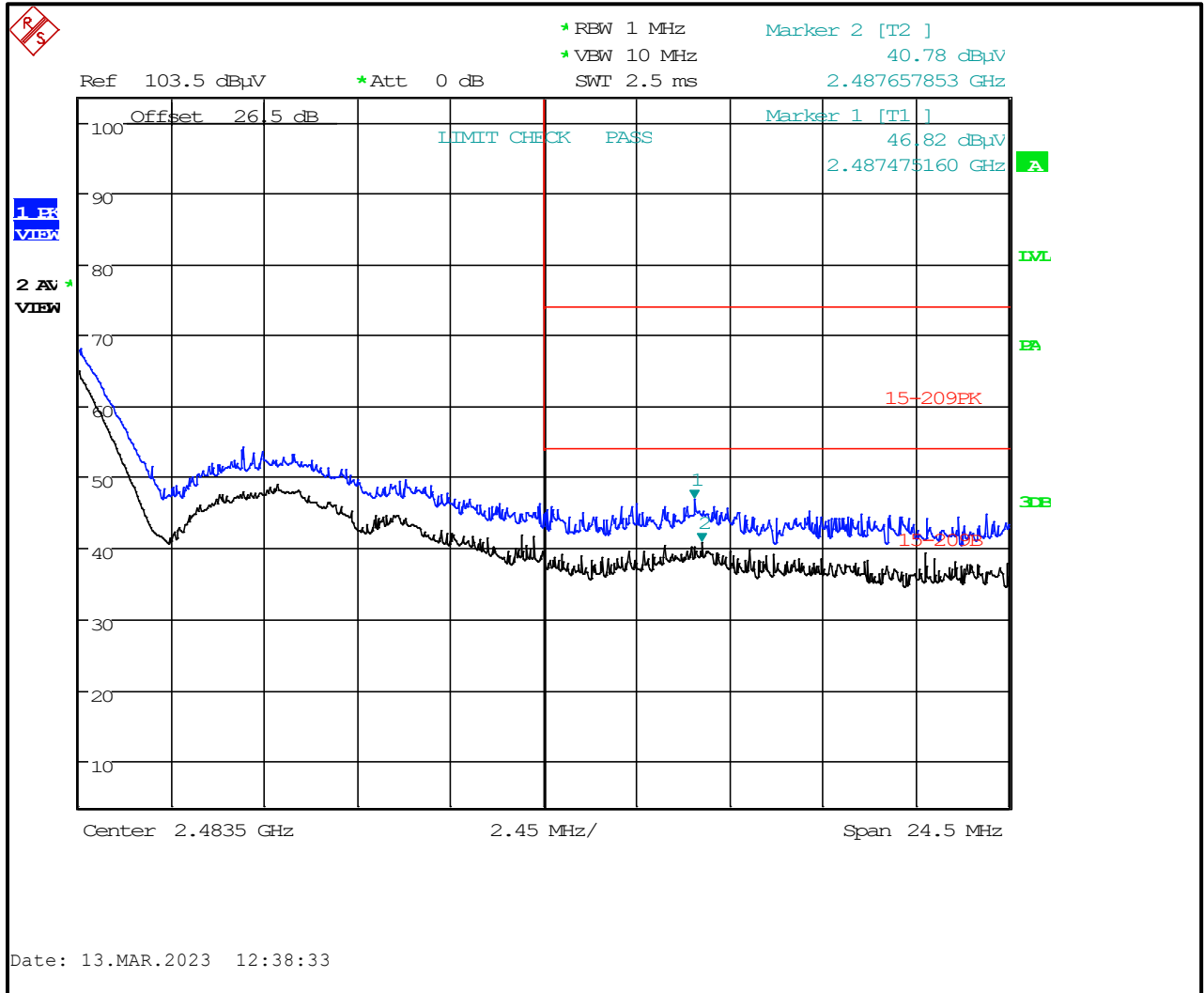
Plot 4-2: Upper Band Edge – 802.11b (1.0 Mbps)
