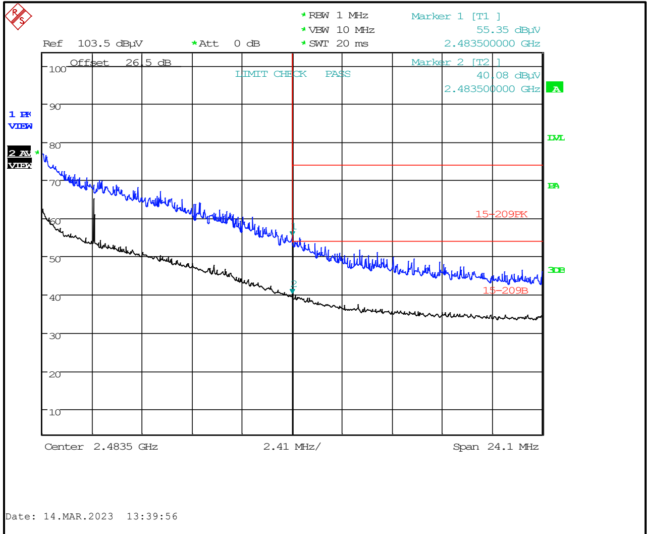
Plot 4-4: Upper Band Edge – 802.11g (12.0 Mbps)
