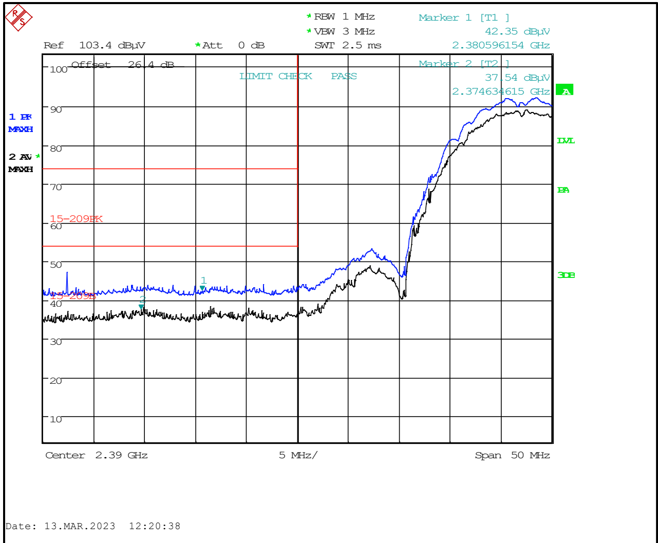
Plot 4-1: Lower Band Edge – 802.11b (1.0 Mbps)
