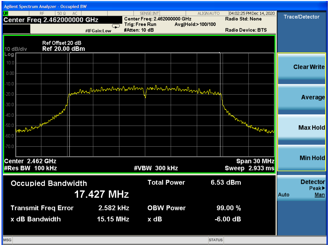
Plot 6-9: 6 dB and 99% Bandwidth – 2462 MHz – 802.11n (65.0 Mbps)
