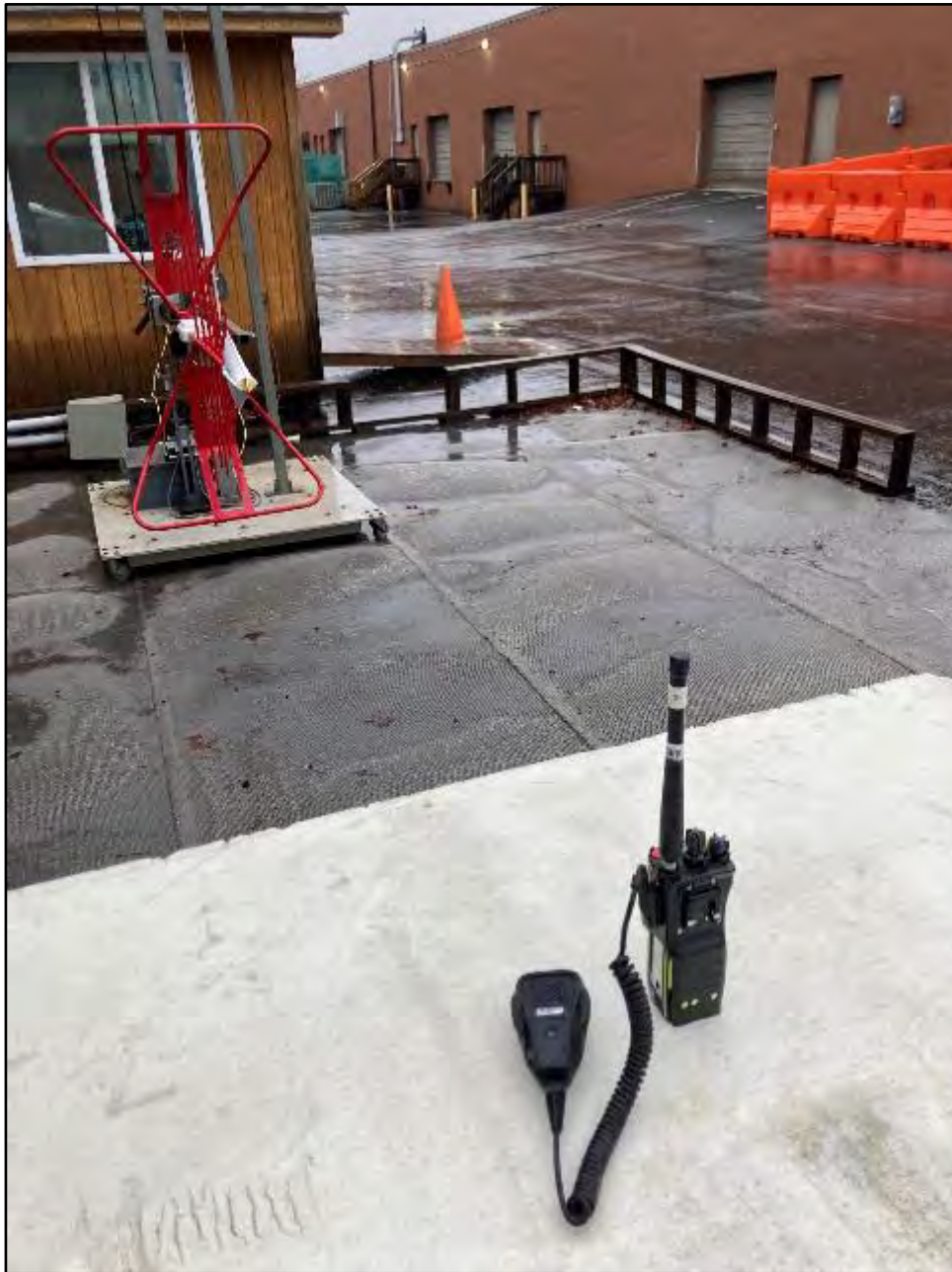
Photograph 2: Radiated Emissions – Back View (Below 1 GHz)
