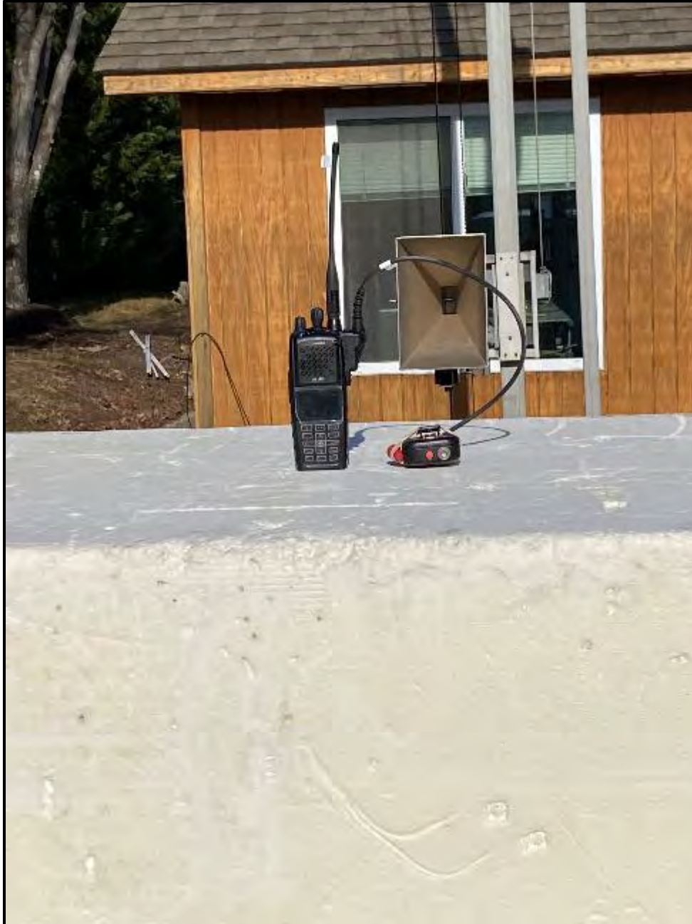
Photograph 1: Radiated Emissions (Spurious/Harmonics) – Front View
