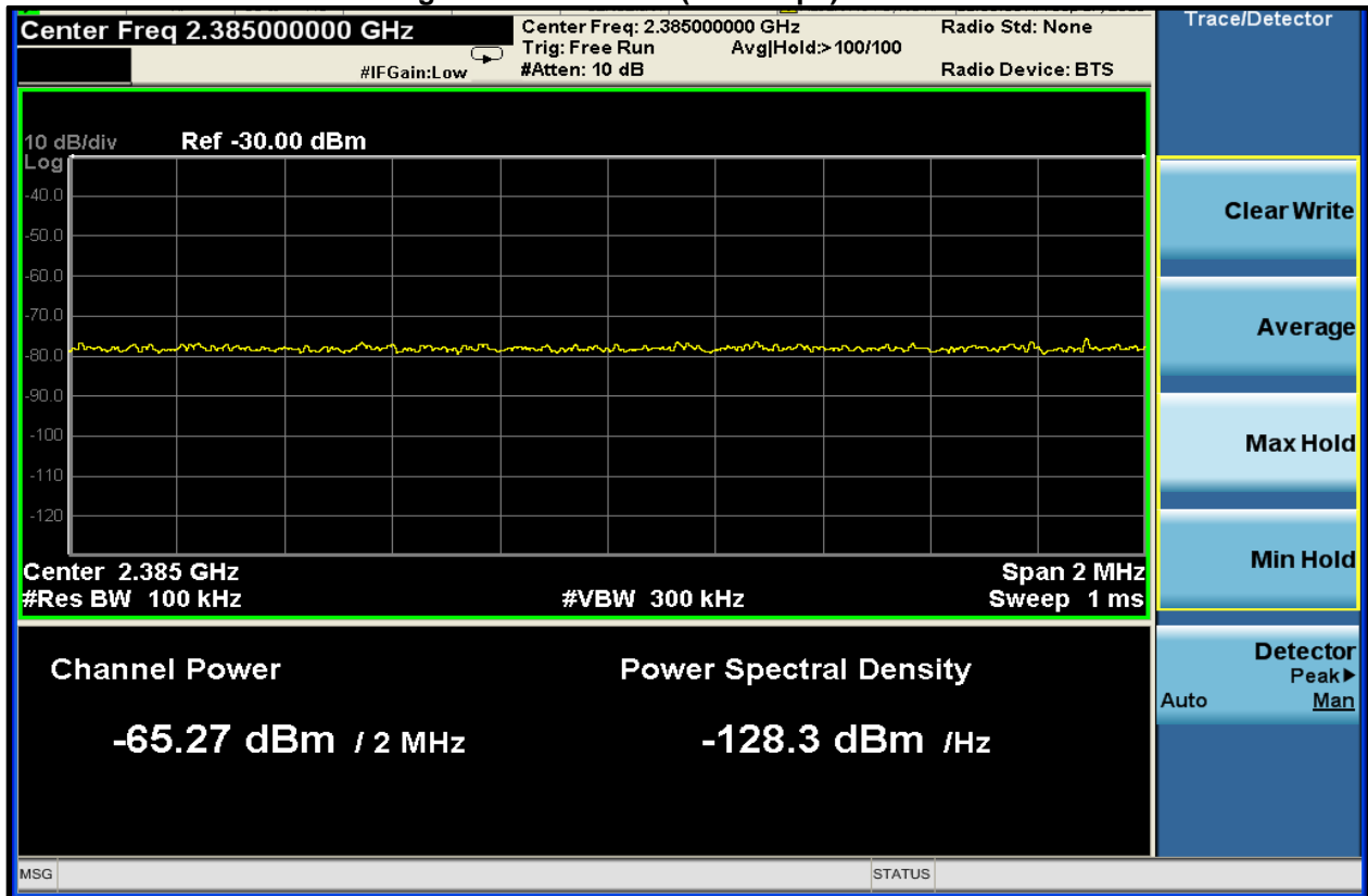
Plot 4-2: Lower Band Edge – Peak – 802.11 (11.0 Mbps)
