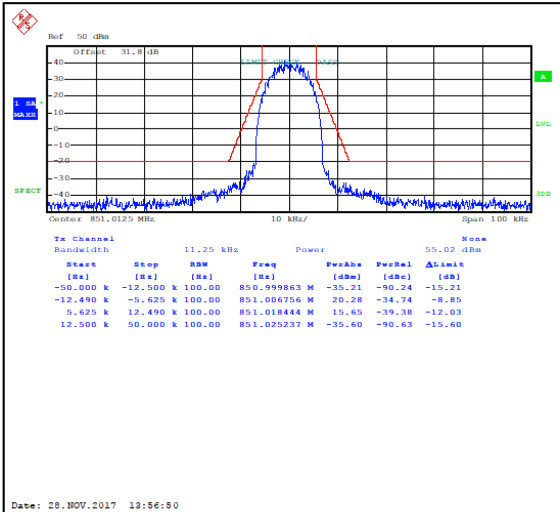
Plot 7-17: Occupied Bandwidth – 851.0125 MHz; WCQPSK; Mask D
