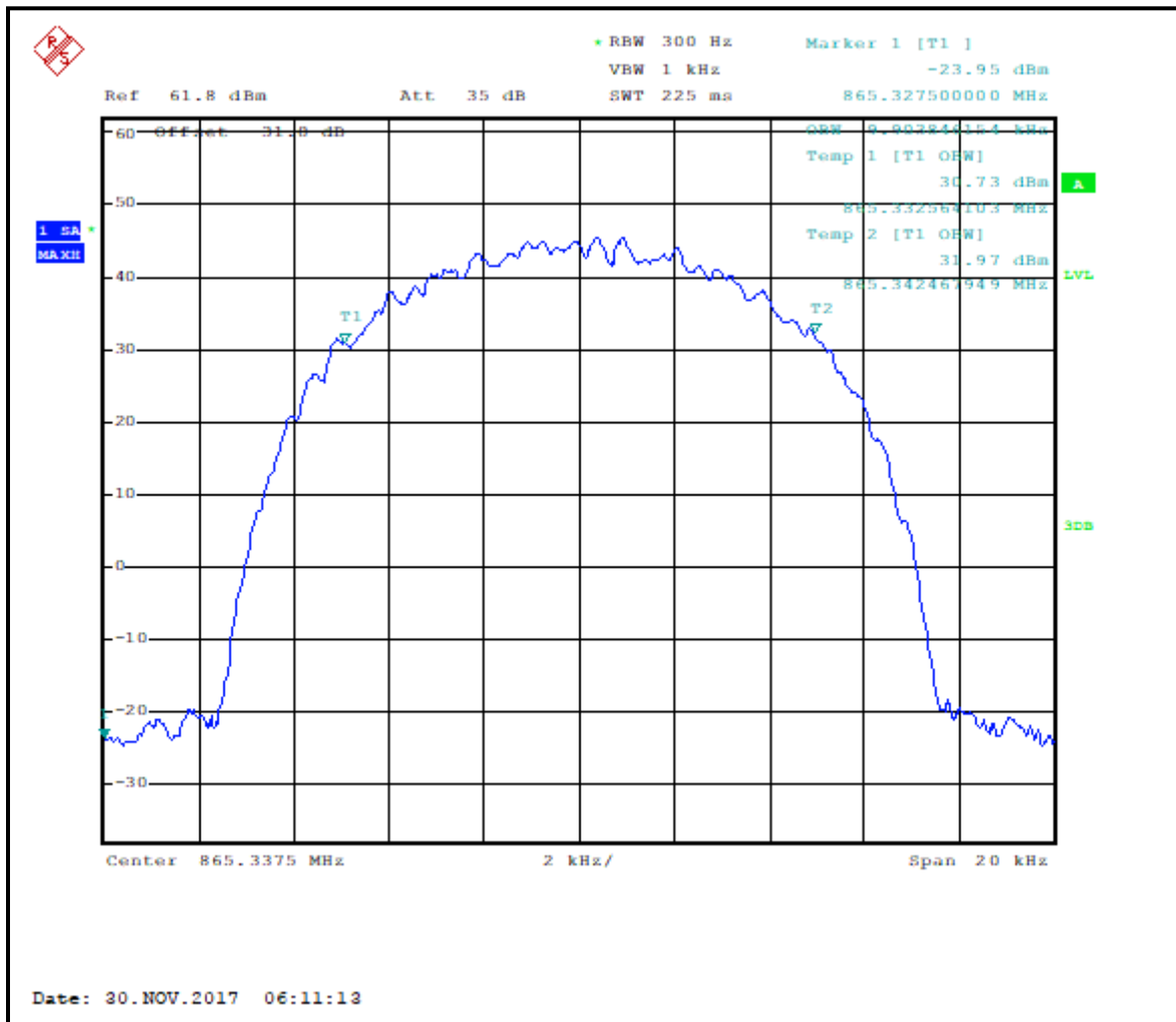
Plot 7-33: Occupied Bandwidth – 865.3375 MHz; HDQPSK; 99% BW
