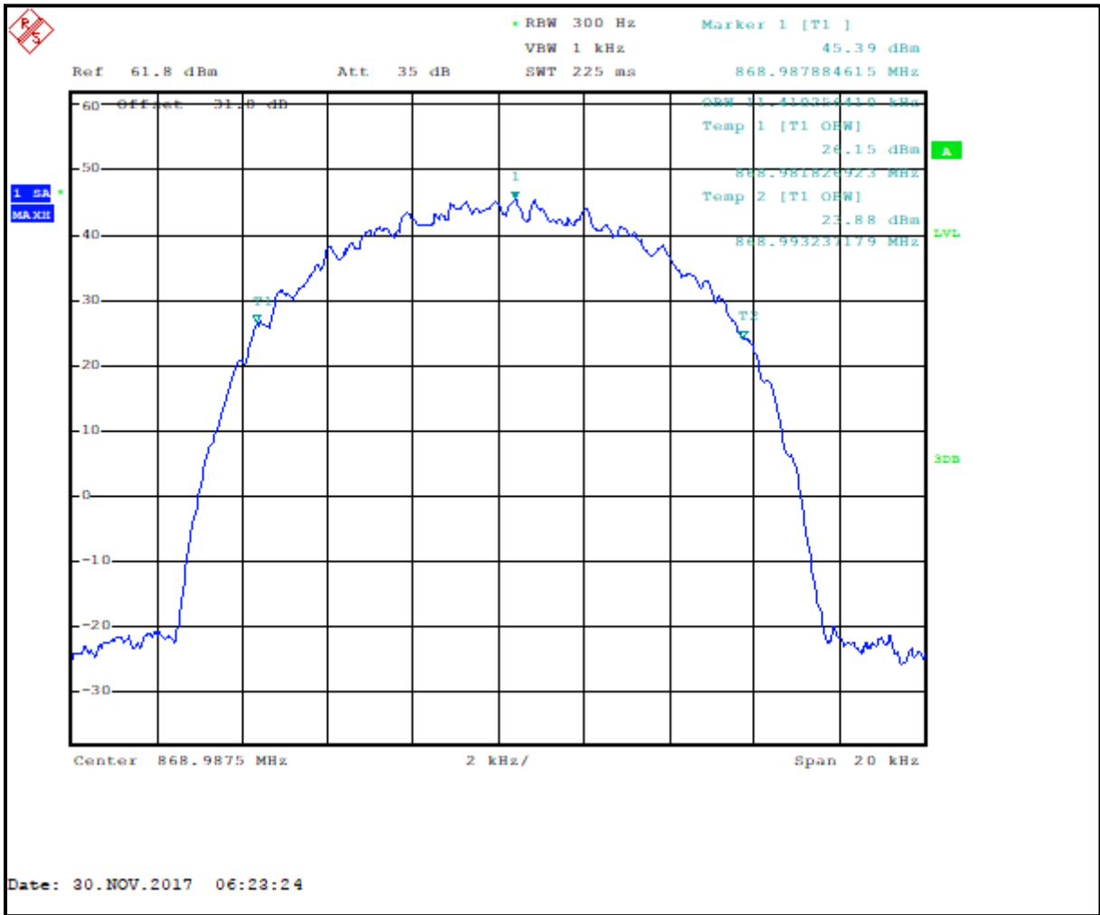
Plot 7-48: Occupied Bandwidth – 868.9875 MHz; HDQPSK; 20 dB BW
