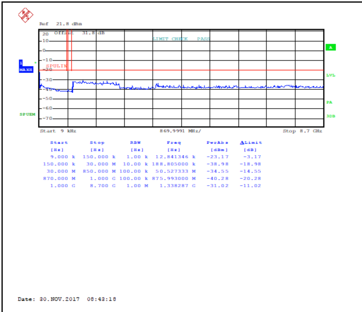
Plot 5-1: Conducted Antenna Spurious Emissions – 851.0125 MHz; C4FM
