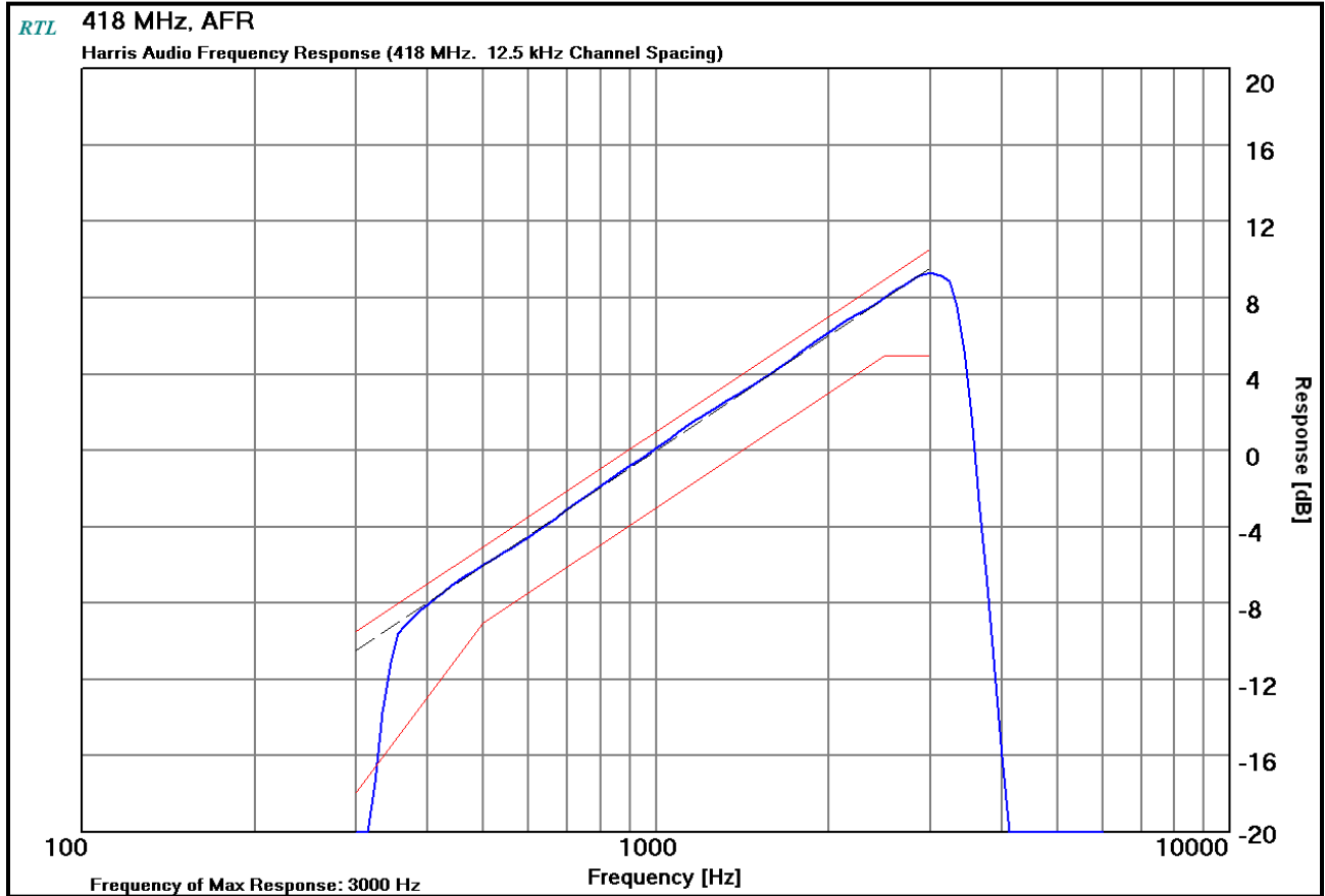
Plot 9-1: Modulation Characteristics - Audio Frequency Response - 418 MHz
