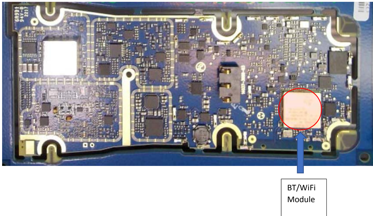
Bottom side of PWB without shields, BT/WiFi module location
