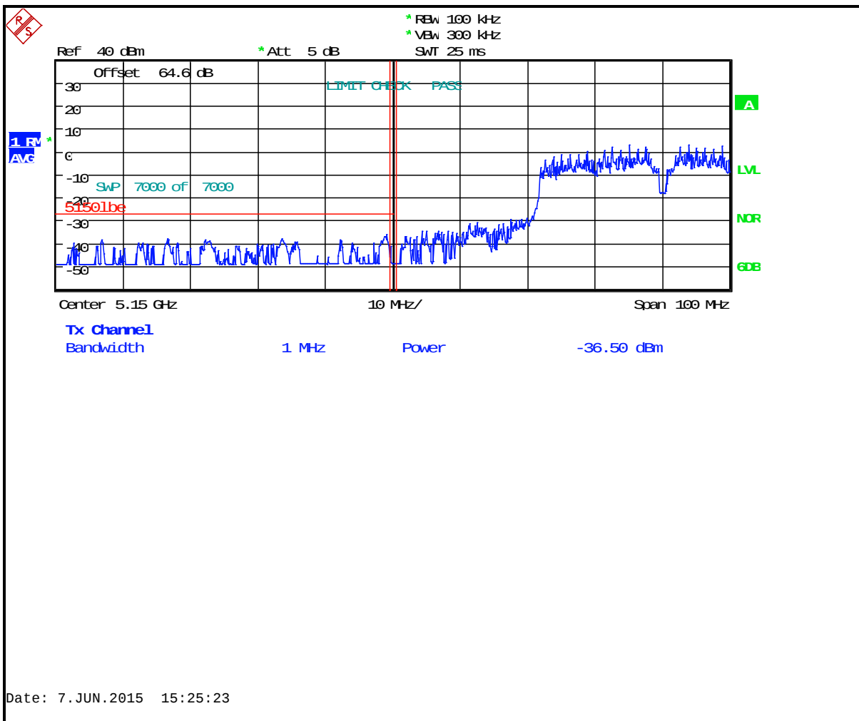
Plot 6-8: Lower Band Edge: Measurement Channel 36 (5180 MHz, 40 MHz BW, 802.11n, Average)
