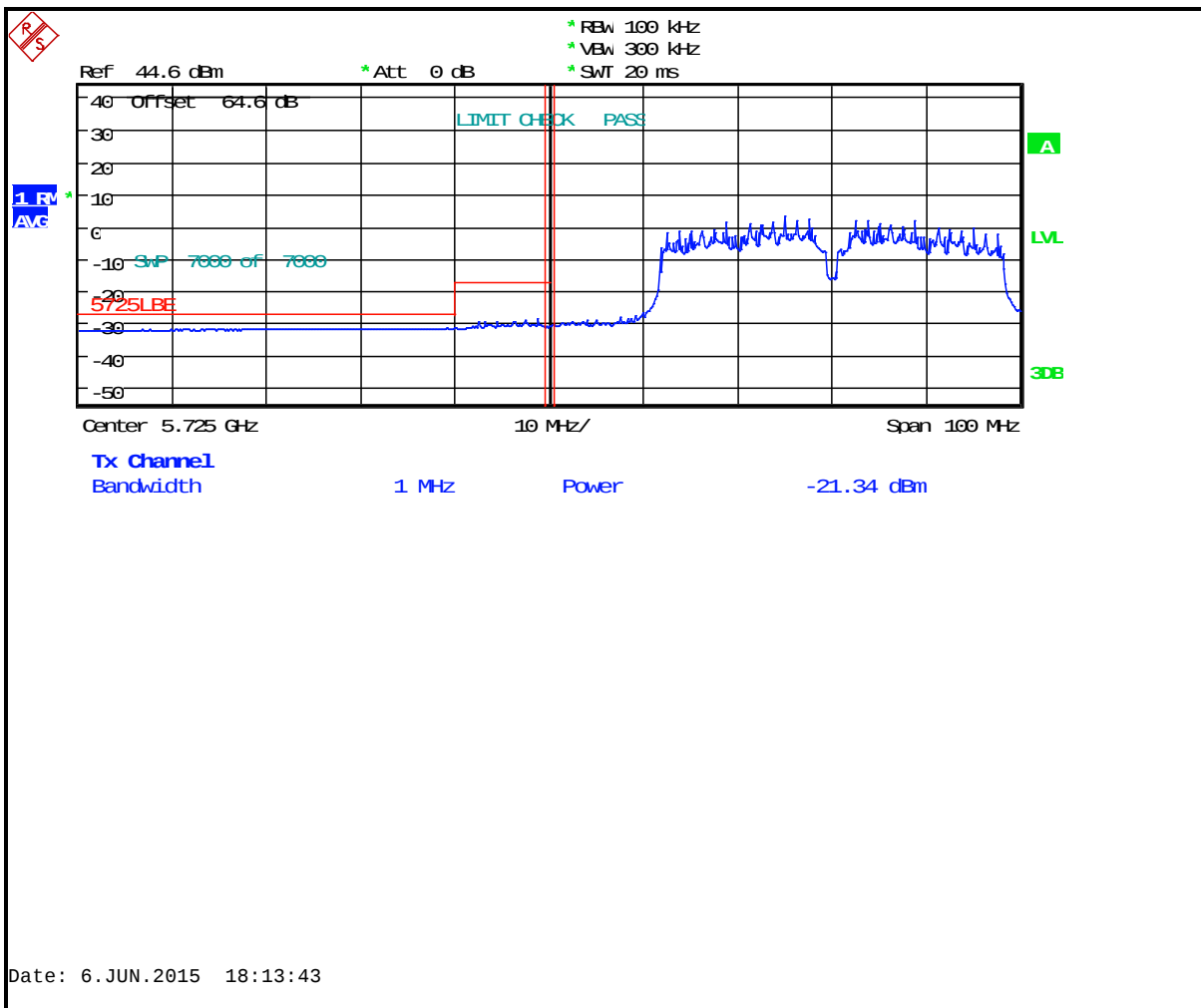
Plot 6-16: Lower Band Edge: Measurement Channel 149 (5745 MHz, 40 MHz BW, 802.11n, Average)
