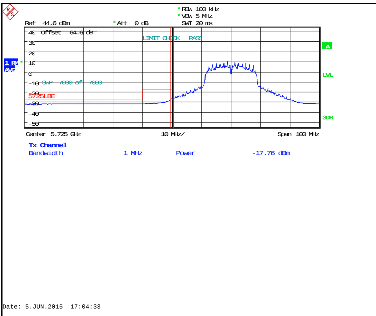
Plot 6-10: Lower Band Edge: Measurement Channel 149 (5745 MHz, 802.11a, Average)
