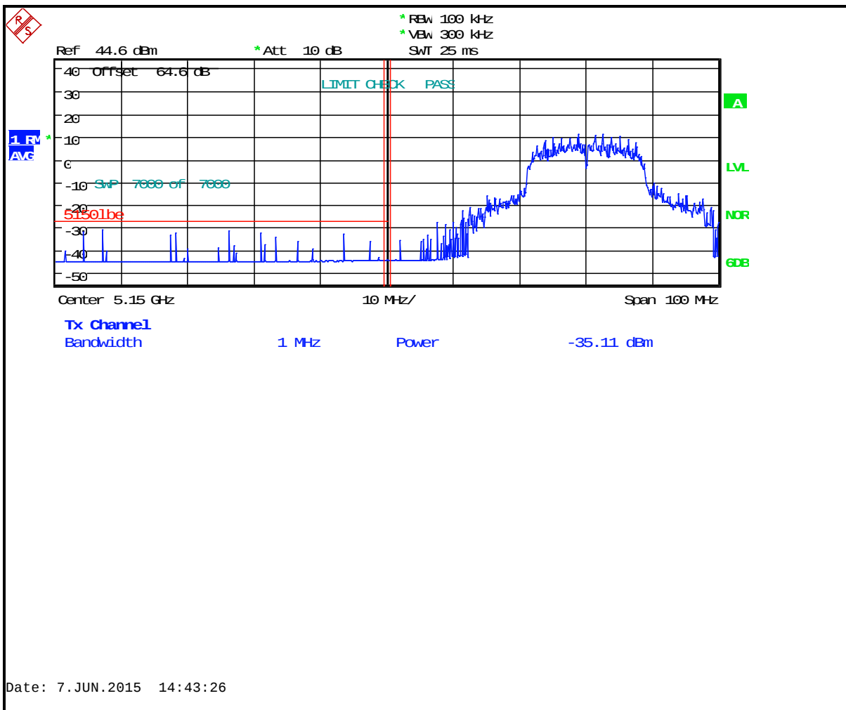
Plot 6-4: Lower Band Edge: Measurement Channel 36 (5180 MHz, 802.11n, Average)
