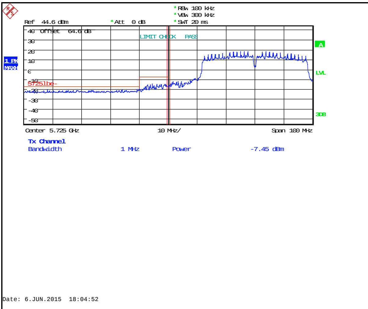
Plot 6-13: Lower Band Edge: Measurement Channel 149 (5745 MHz, 40 MHz BW, 802.11a, Peak)
