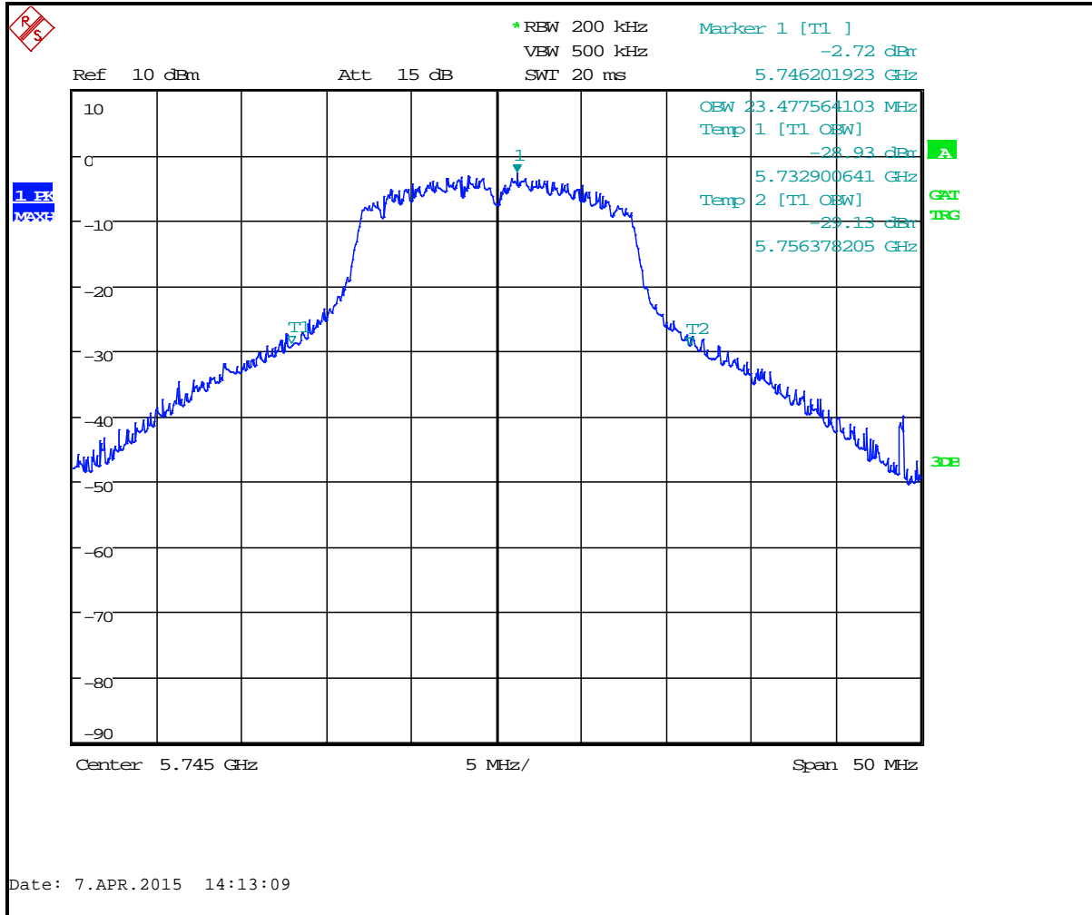
Plot 8-12: 26 dB Bandwidth Channel 149 (TX Frequency 5745 MHz) - 802.11n
