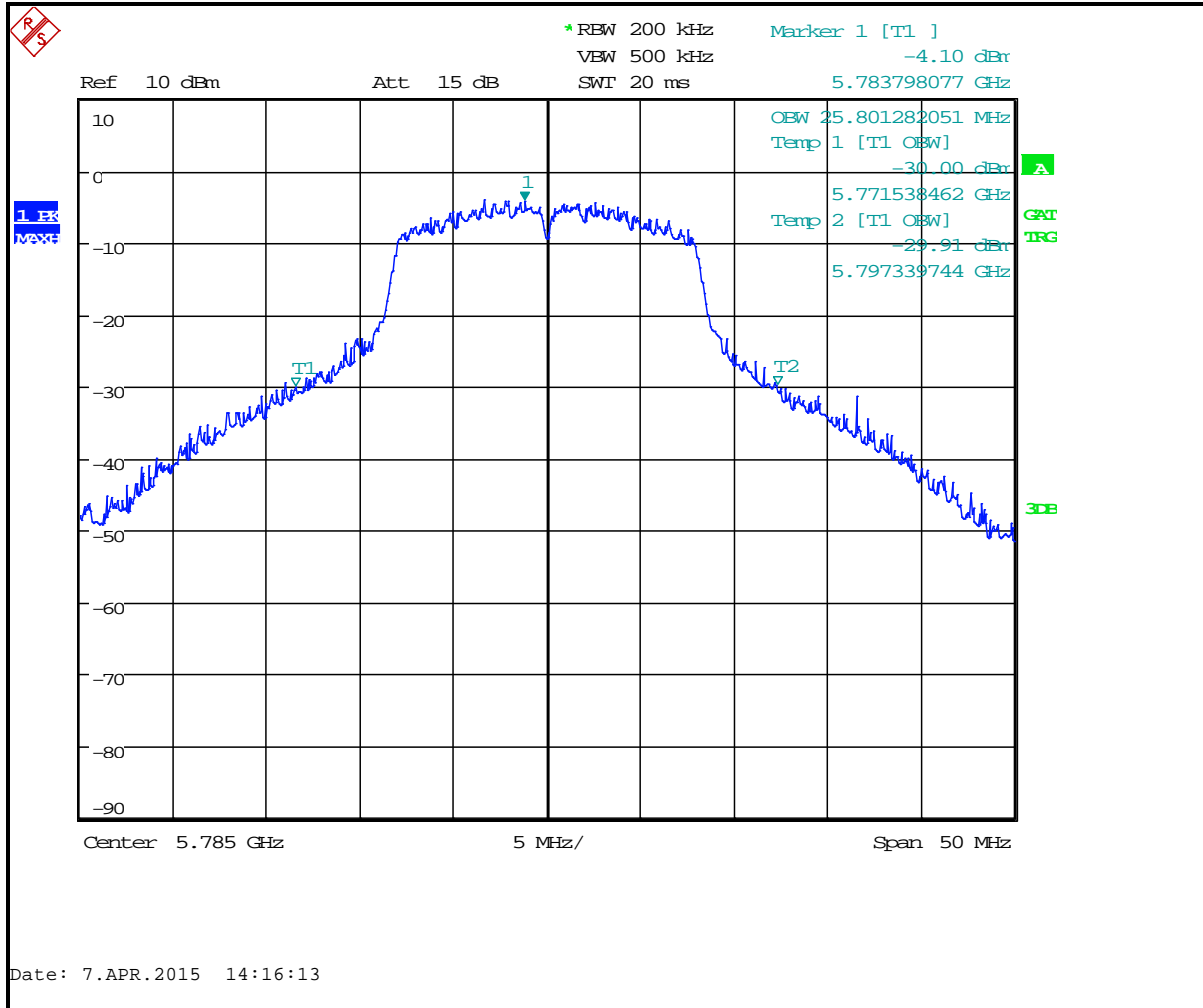
Plot 8-13: 26 dB Bandwidth Channel 157 (TX Frequency 5785 MHz) - 802.11n
