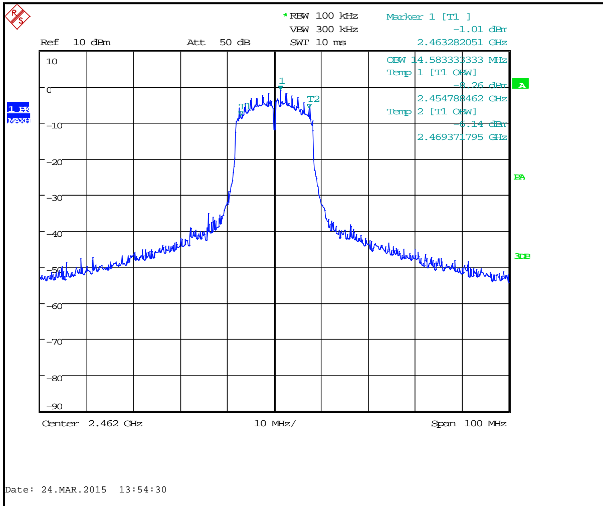
Plot 6-9: 6 dB Bandwidth Channel 11 (TX Frequency 2462 MHz-20 MHz BW) - 802.11n
