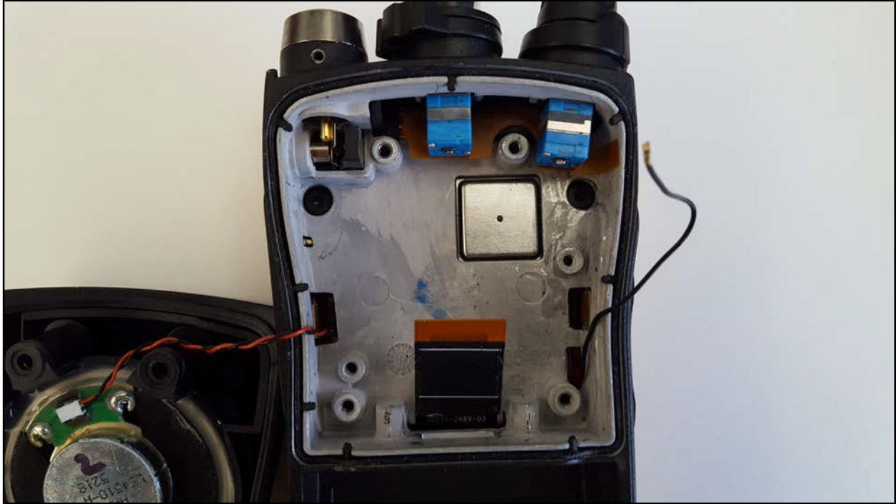
Rear Cover and Expansion Board Removed
