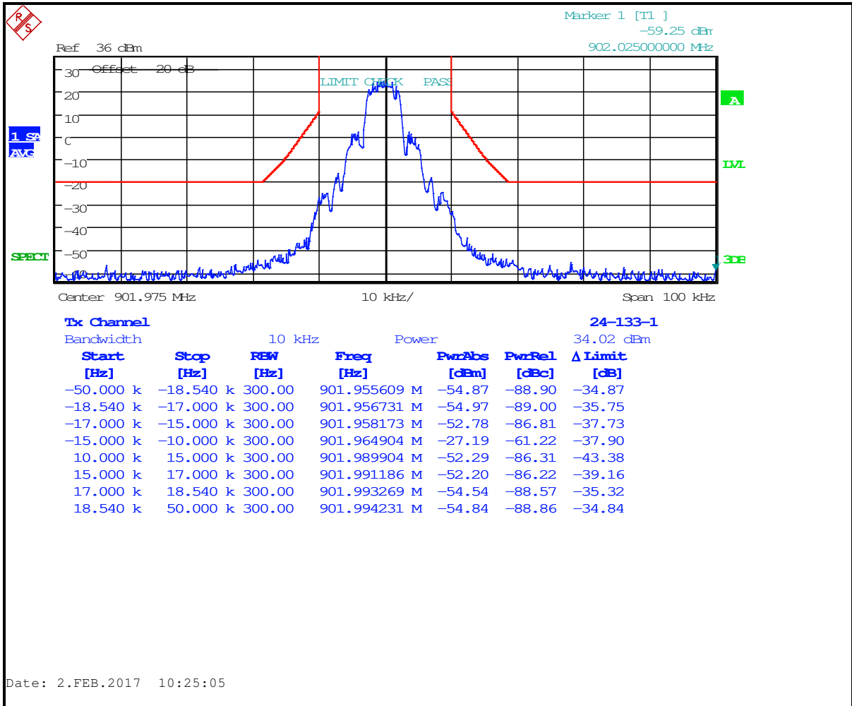
Plot 8-99: Occupied Bandwidth – 901.9750 MHz; 2-Level FSK 4800 XNB; Mask 24.133(1)
