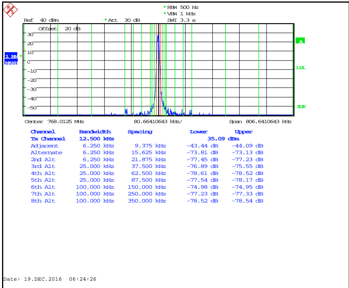
Plot 6-1: Adjacent Channel Power - 768.0125 MHz; Analog Mode (9.375 kHz - 350 kHz)
