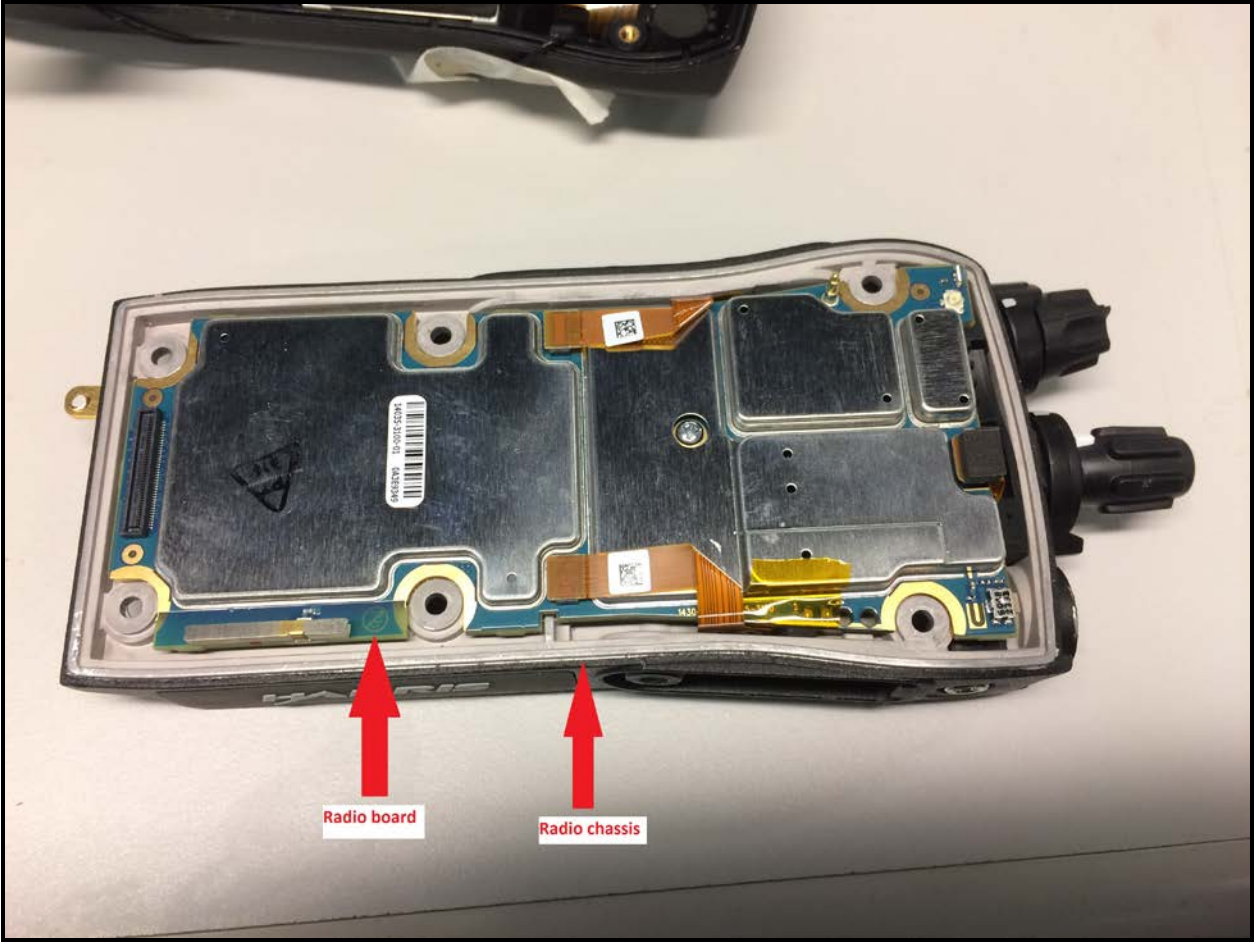
XL-185P PCB in Chassis
