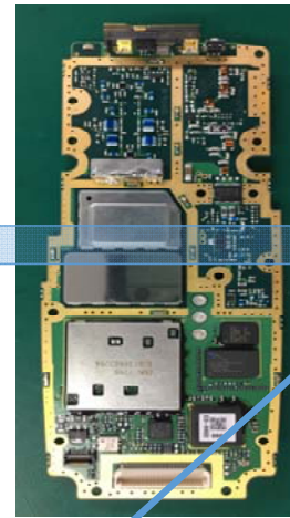
RF board
