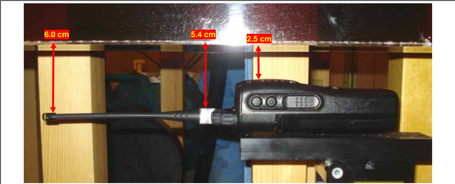
Face-held test setup - Antenna 1
