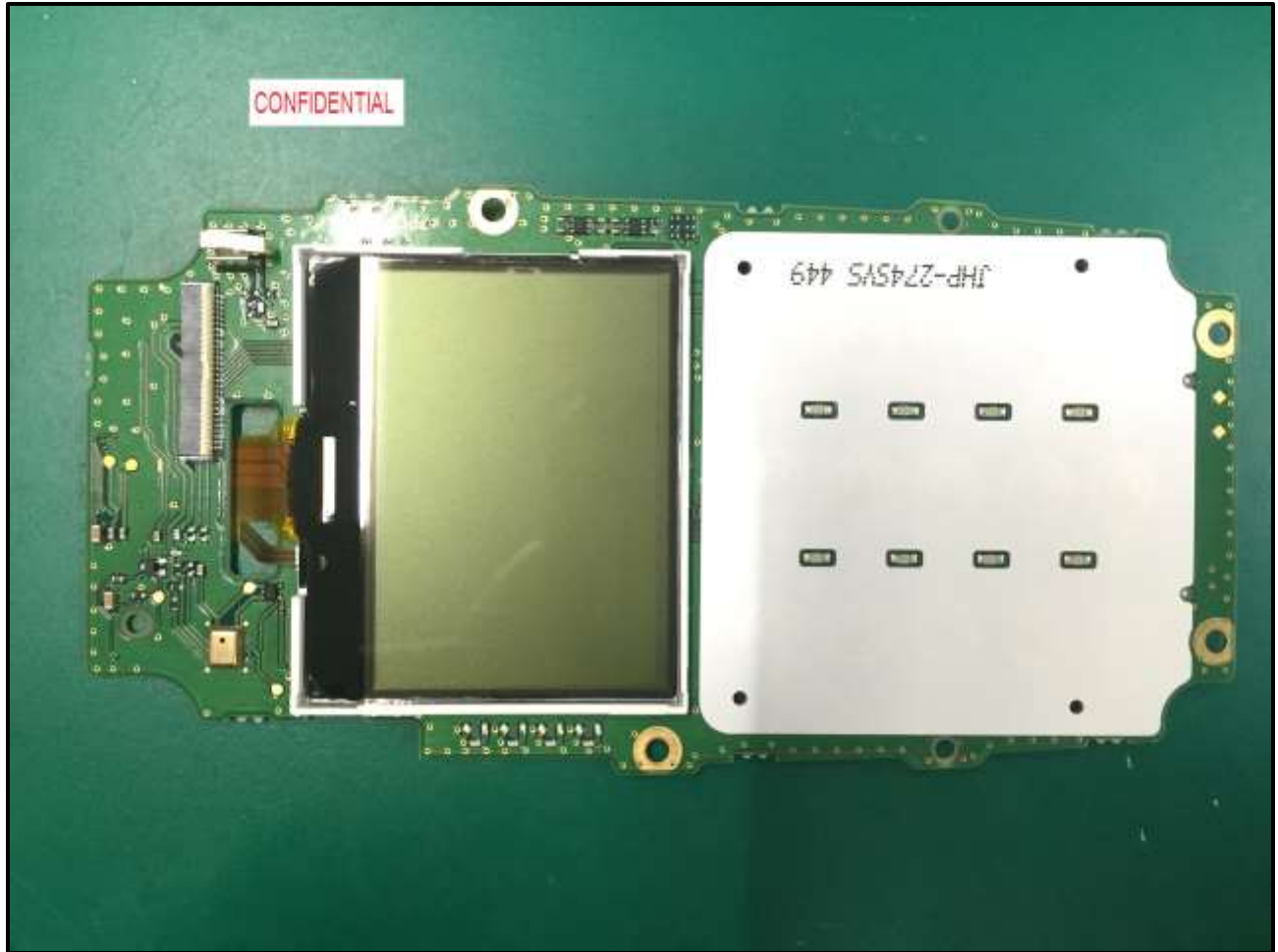
Photograph 12: IF Board with Keypad and Display – Top View
