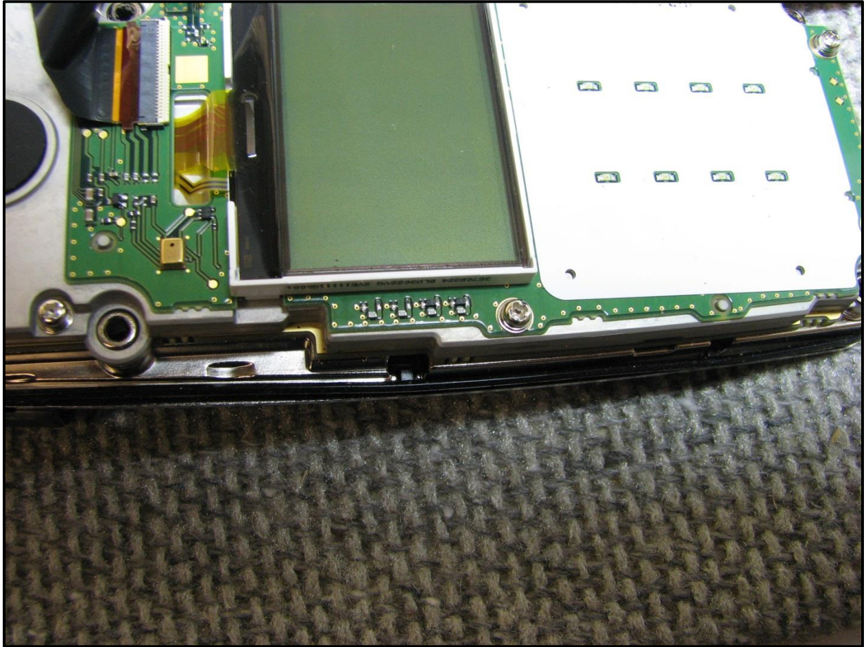
Photograph 15: IF Board View 2
