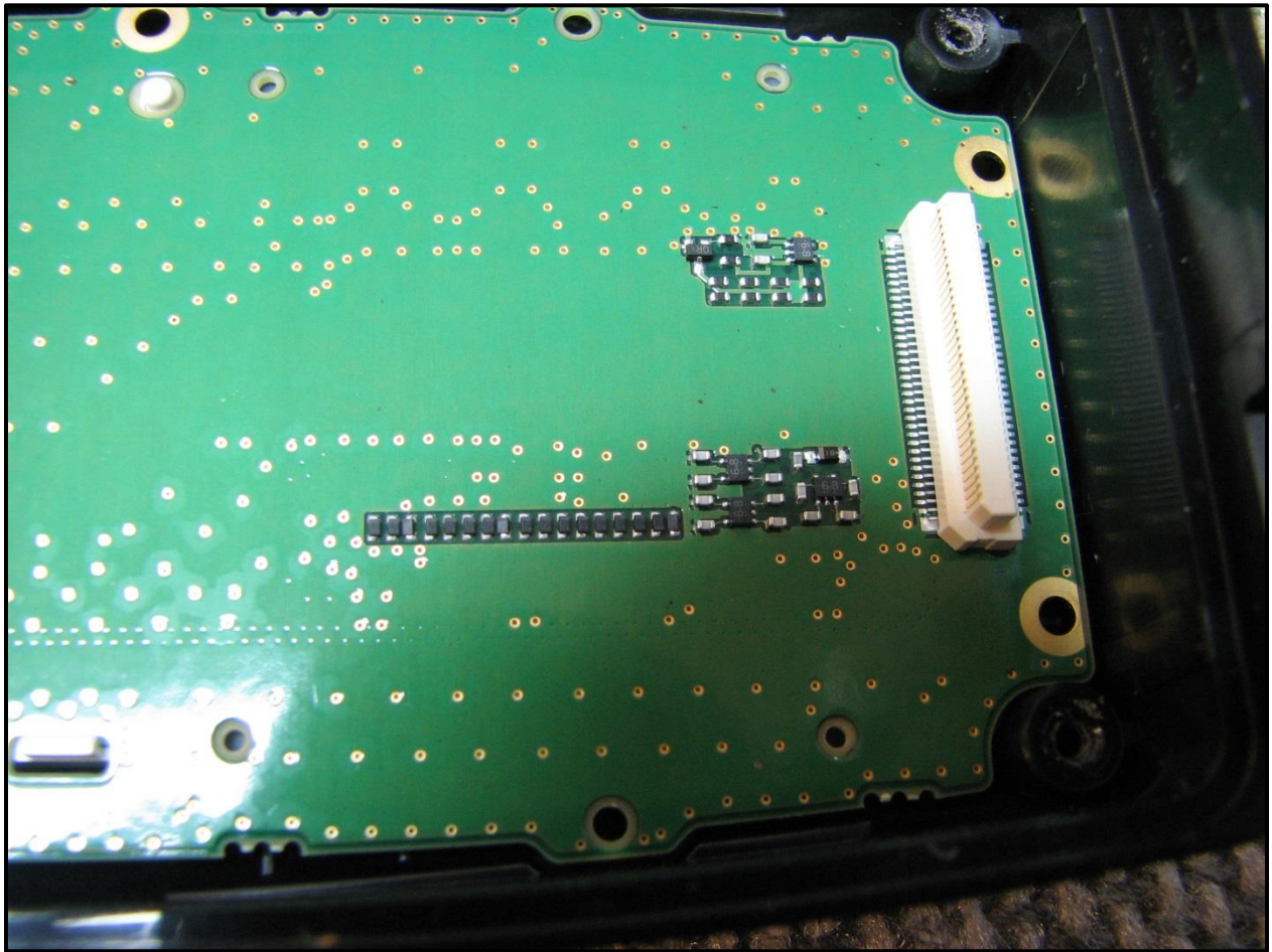
Photograph 18: IF Board View 5
