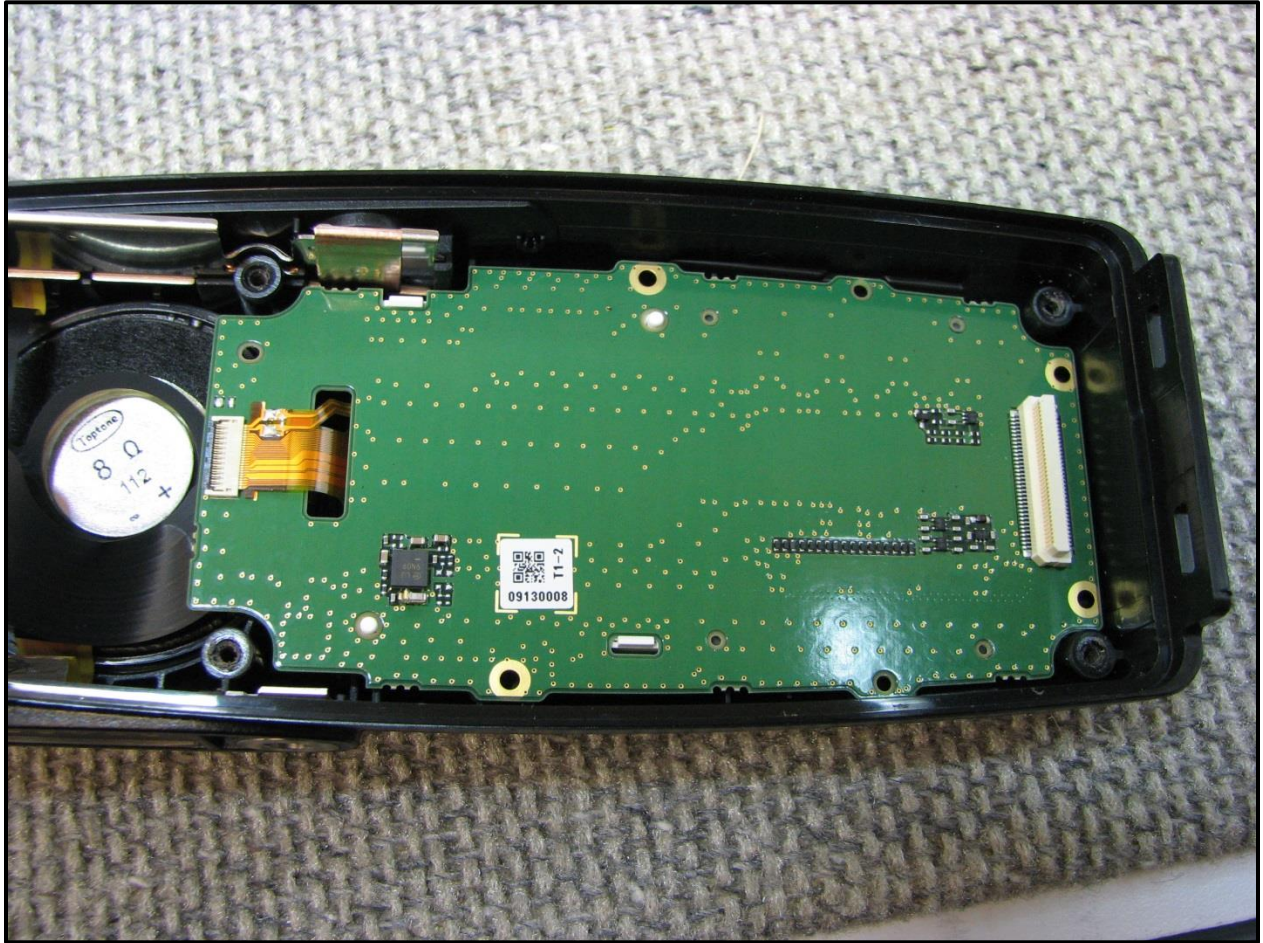
Photograph 19: IF Board View 6
