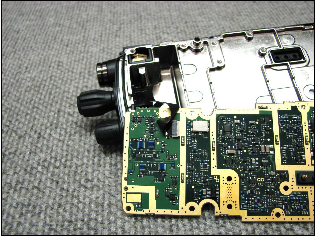
Photograph 24: Main Board Back View 2
