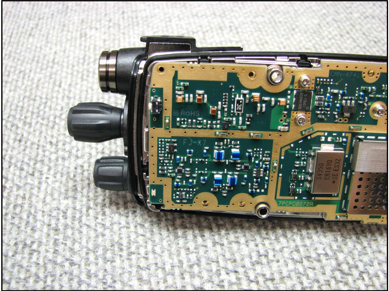
Photograph 20: Main Board View 1
