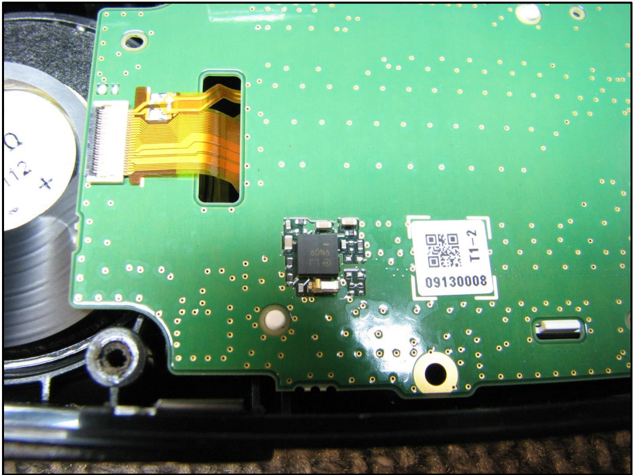
Photograph 17: IF Board View 4
