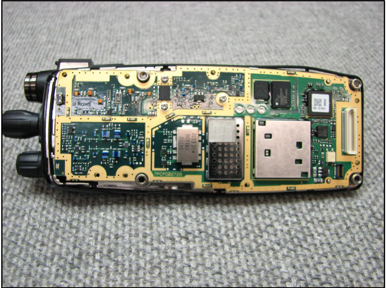
Photograph 22: Main Board View 3
