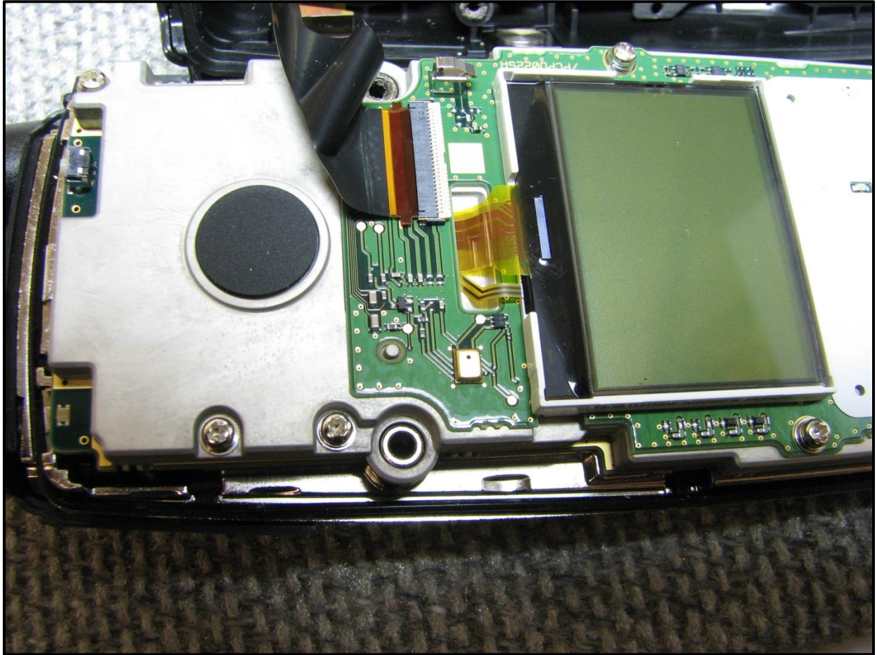
Photograph 14: IF Board View 1
