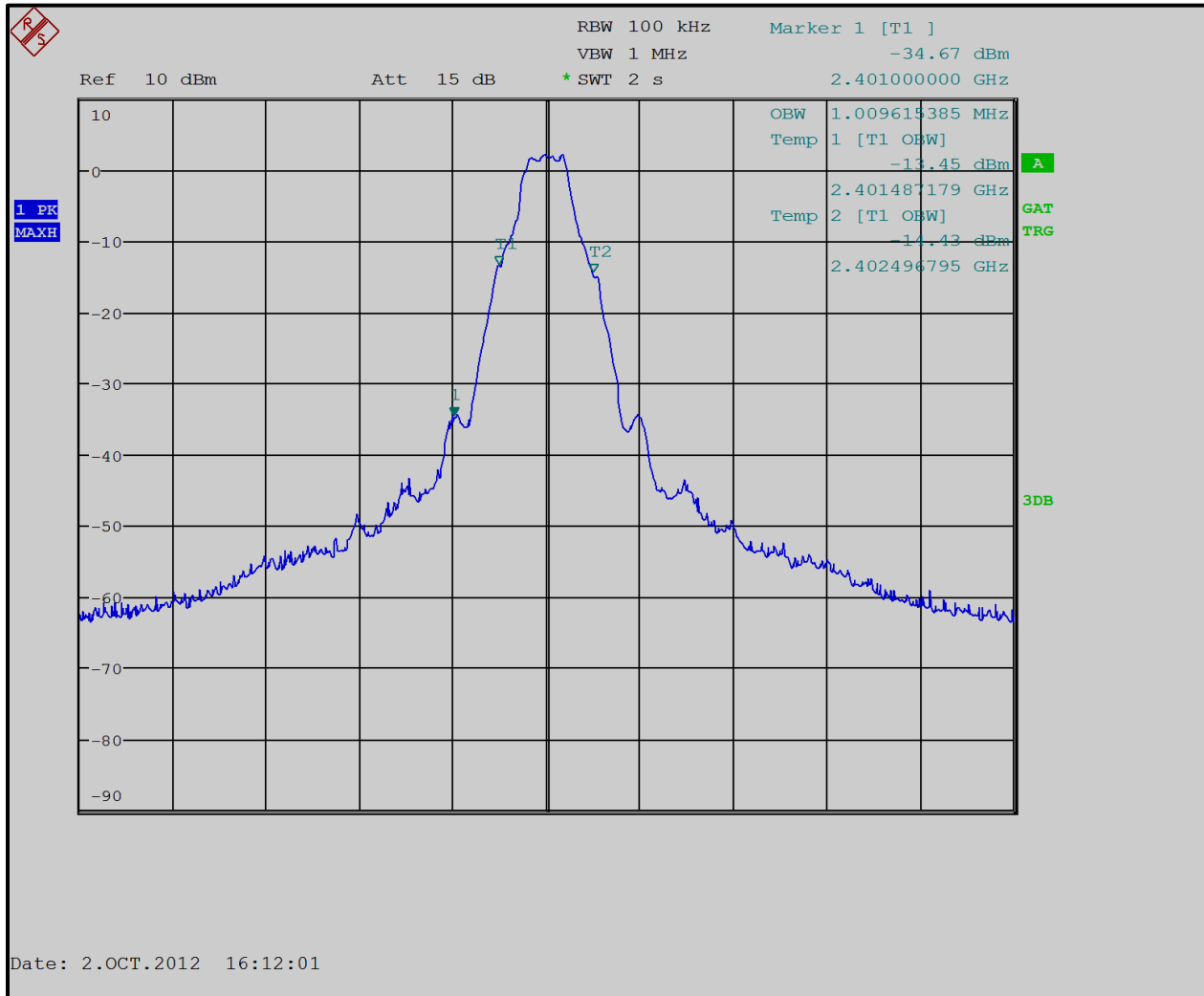
Plot 6-1: 20 dB Bandwidth - 2402 MHz (SDR)
