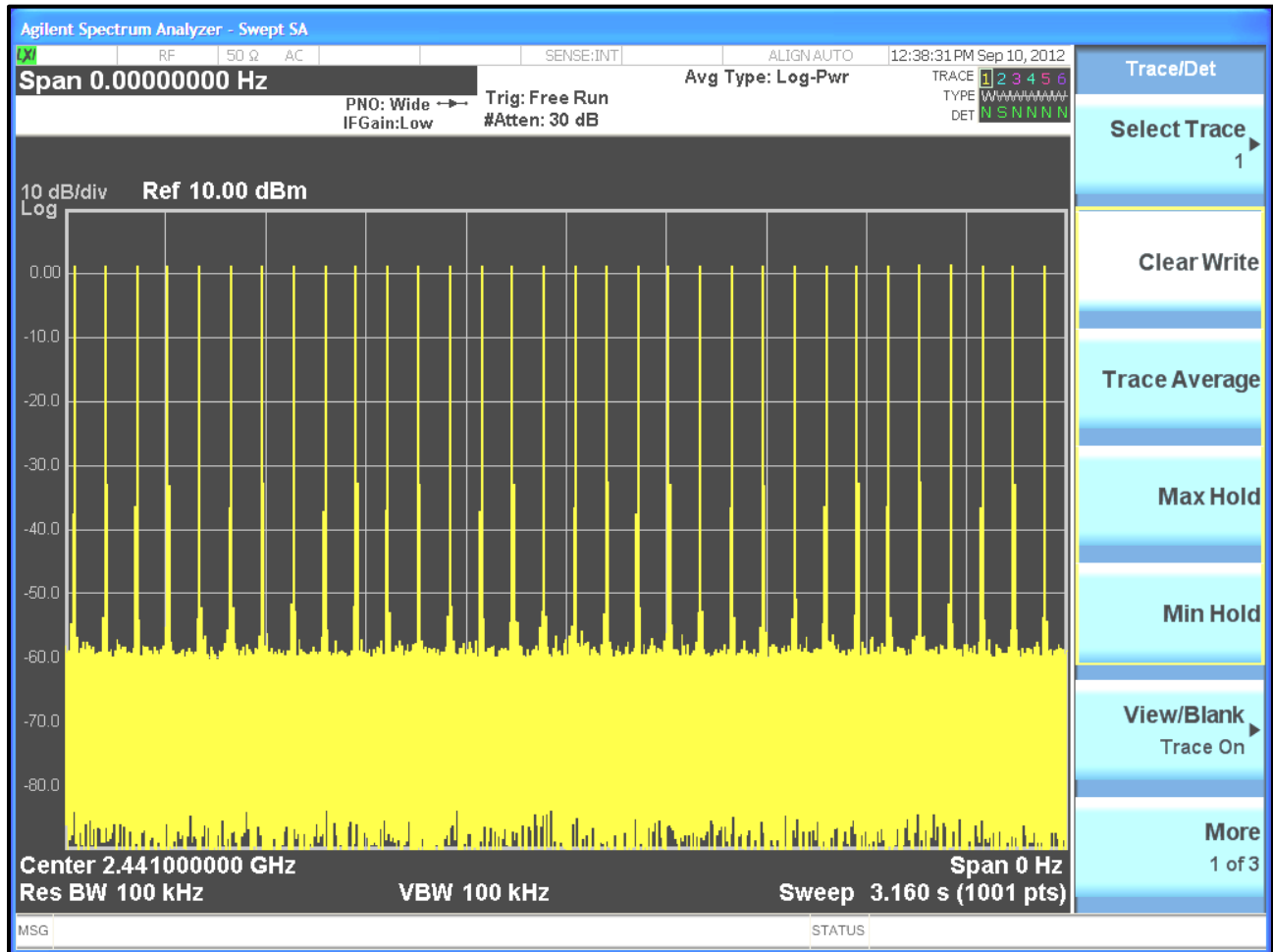
Plot 8-3: Number of Pulses in 3.16 Second Sweep
