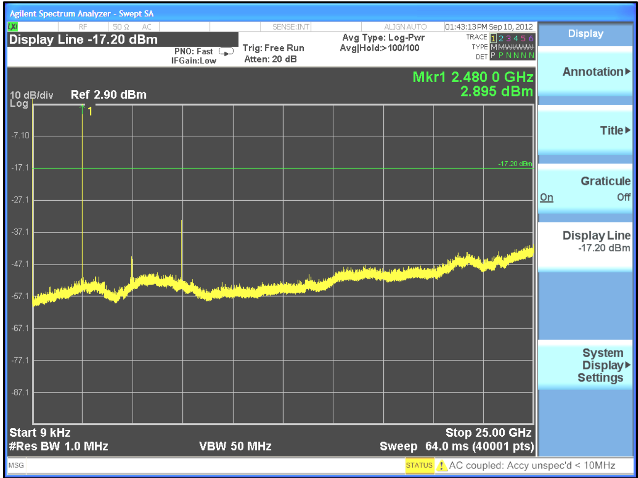
Plot 4-3: Antenna Conducted Spurious TX Frequency - 2480 MHz
