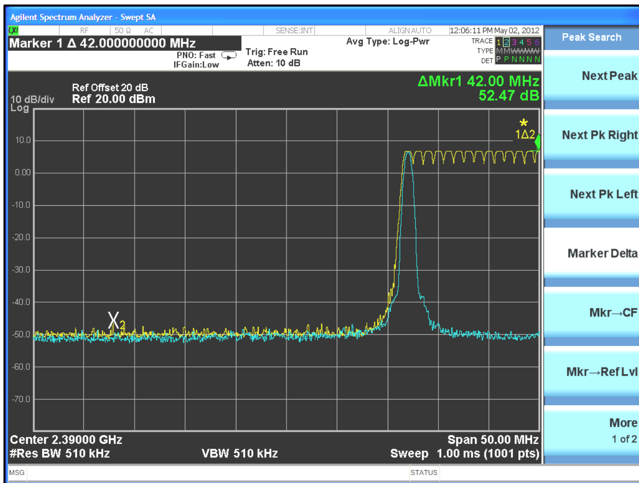
Plot 5-1: Lower Band Edge TX Frequency - 2402 MHz
