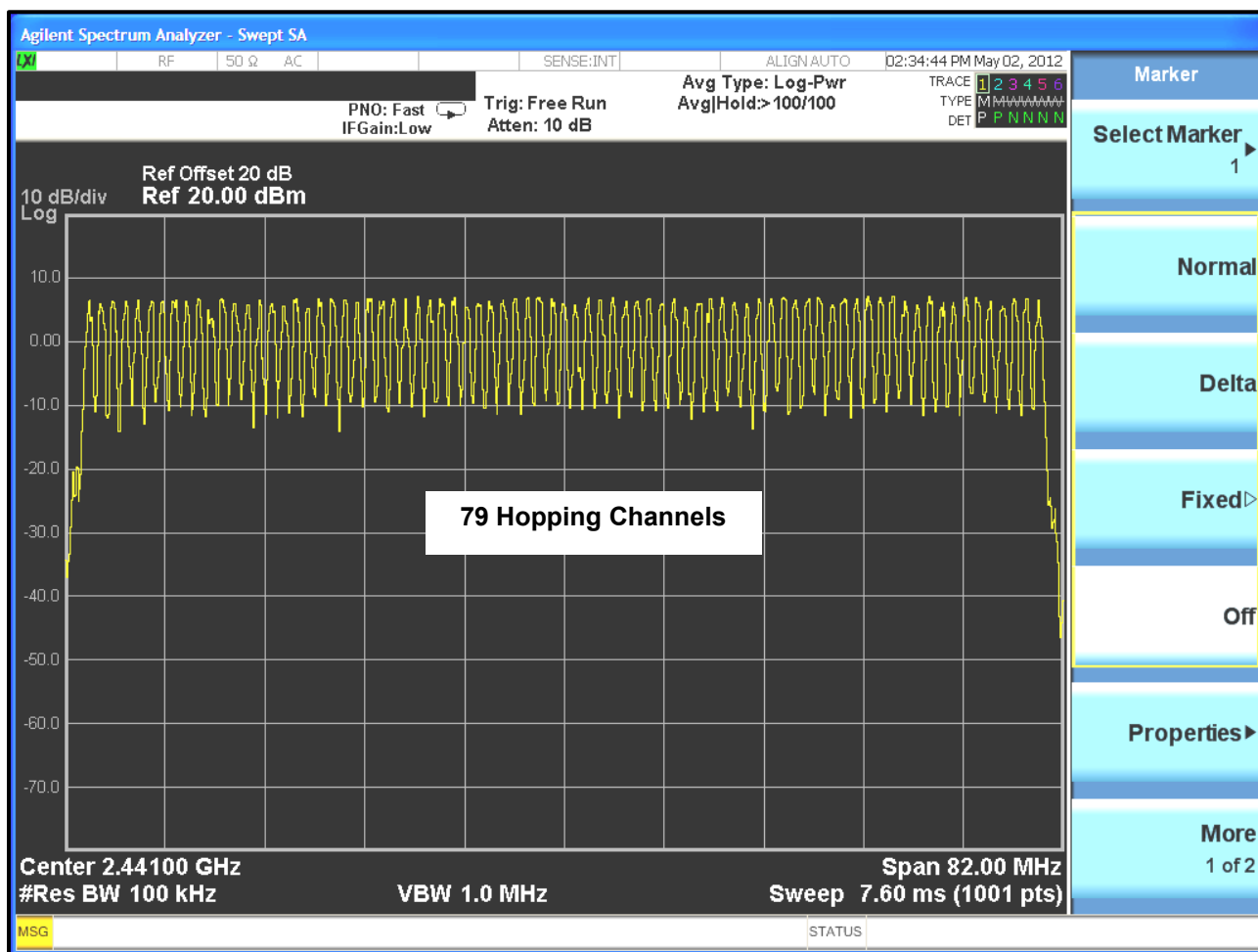
Plot 8-1: Number of Hopping Frequencies (2402 - 2480 MHz)
