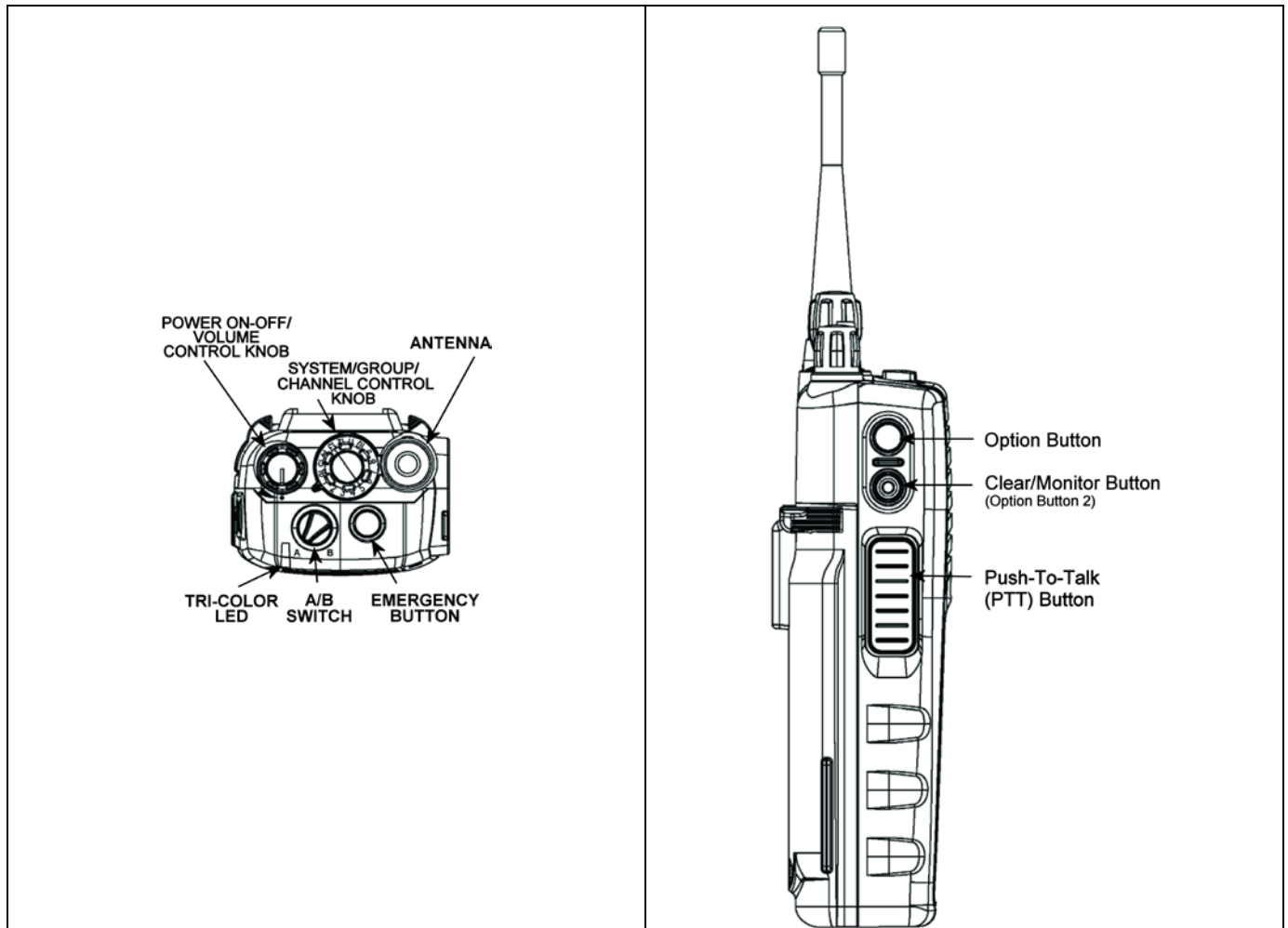
Figure 7-1: Top View
