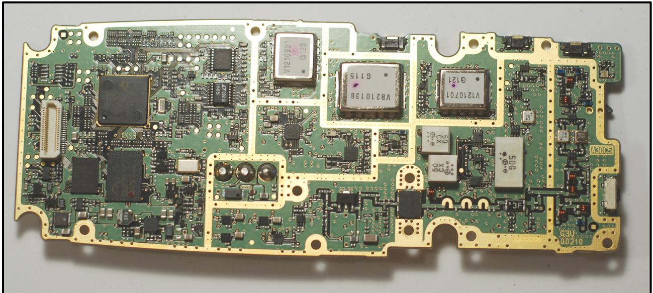
Photograph 17: Main PWB Side 2
