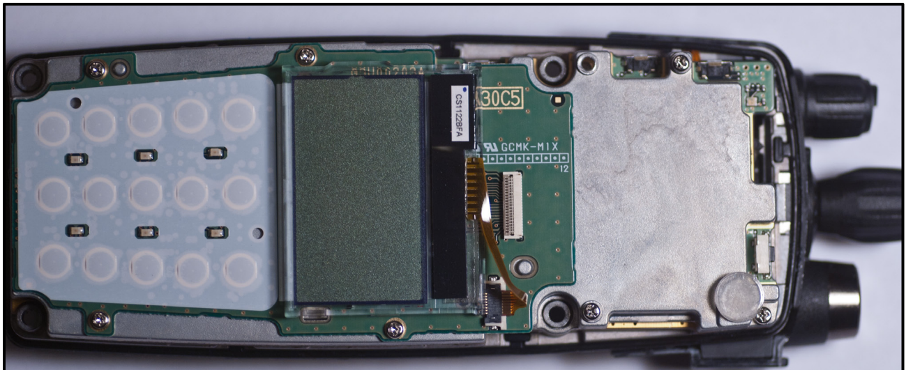
Photograph 18: Interface PWB in Unit
