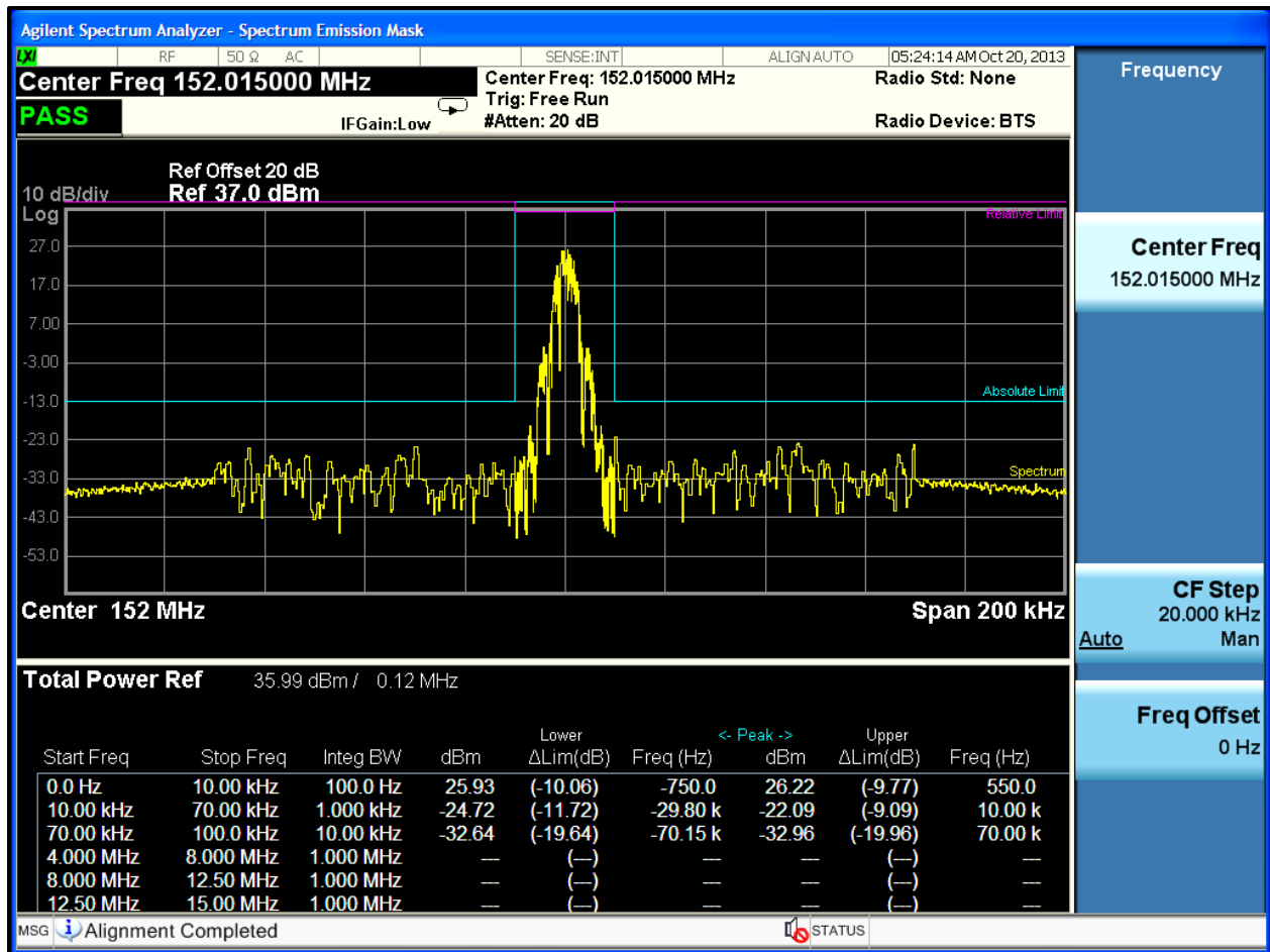
Plot 5-10: Occupied Bandwidth – 152.015 MHz; Mask; 2 Level NB 4800 FSK
