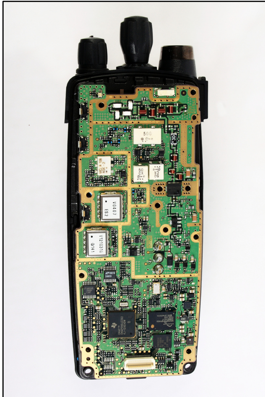
Photograph 18: Main PWB on Casting
