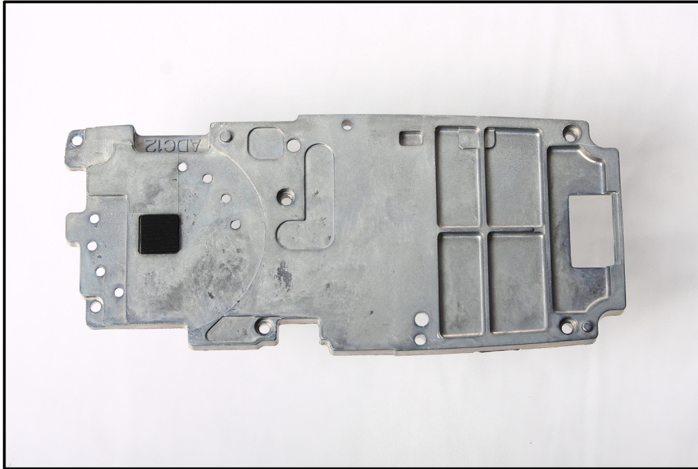
Photograph 14: RF Shield – Side 1
