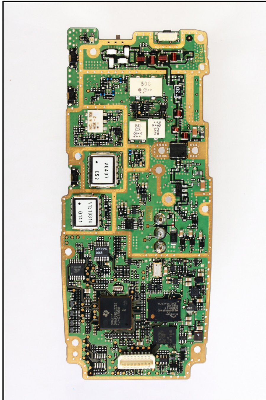
Photograph 16: Main PWB – Front
