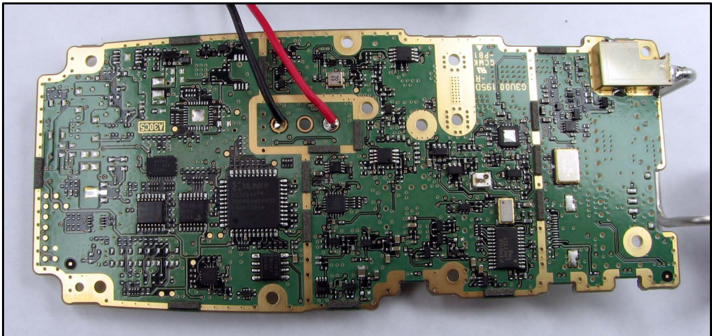
Photograph 10: Main Board Bottom View
