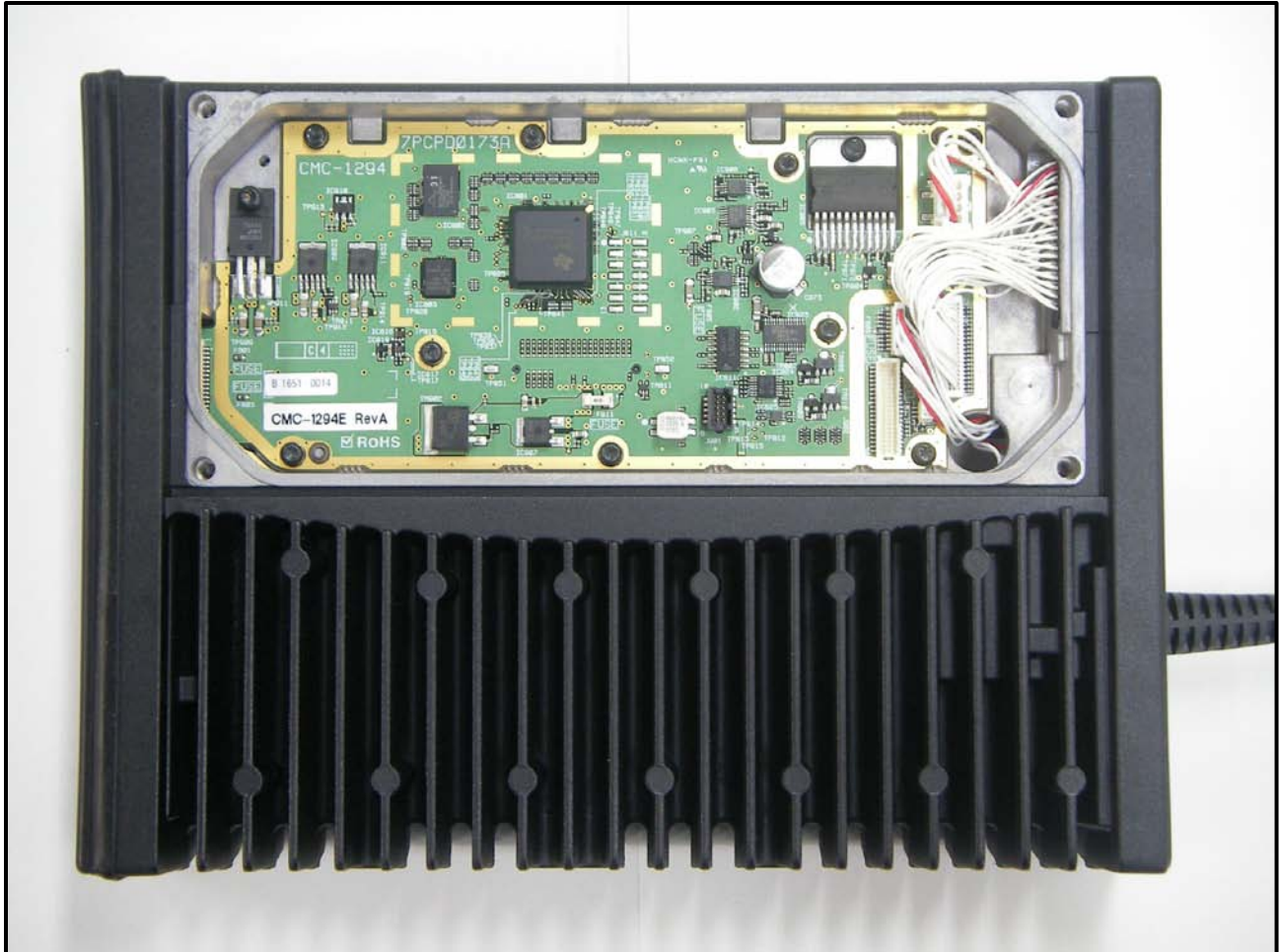
Photograph 19: LB Top Cover Removed
