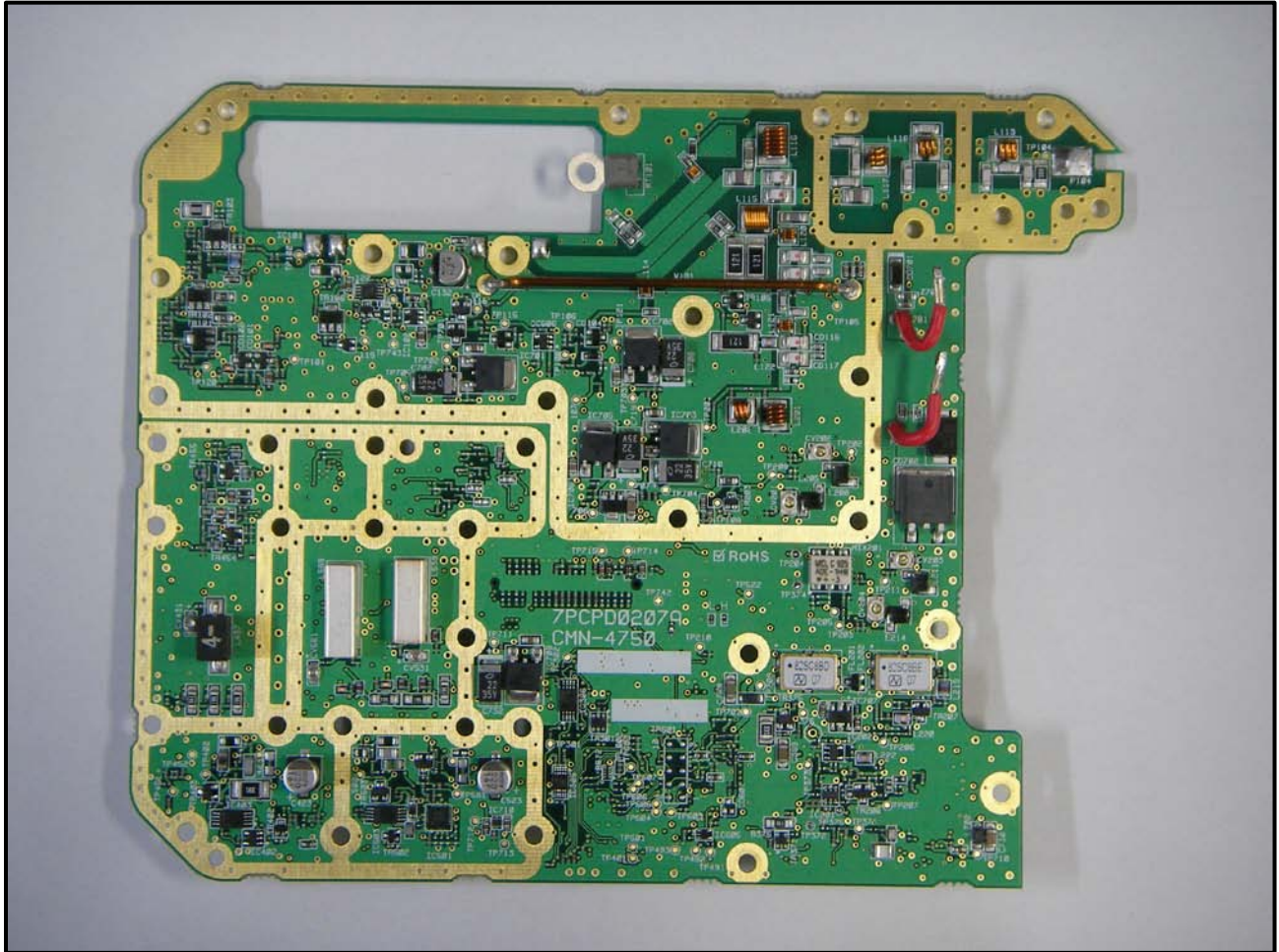
Photograph 24: LB RF Processor Board Component Side
