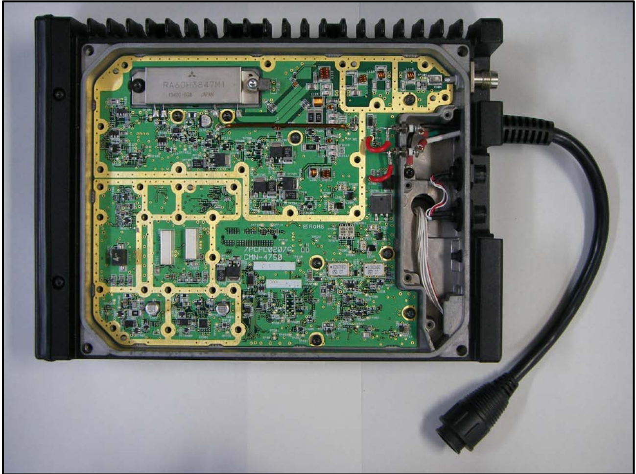
Photograph 21: LB Bottom Cover and Shield Removed
