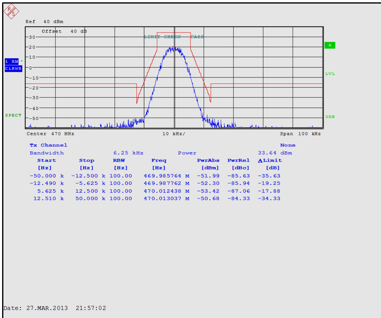
Plot 5-4: Occupied Bandwidth – 470.0000 MHz; H-CPM TDMA (Mask D)
