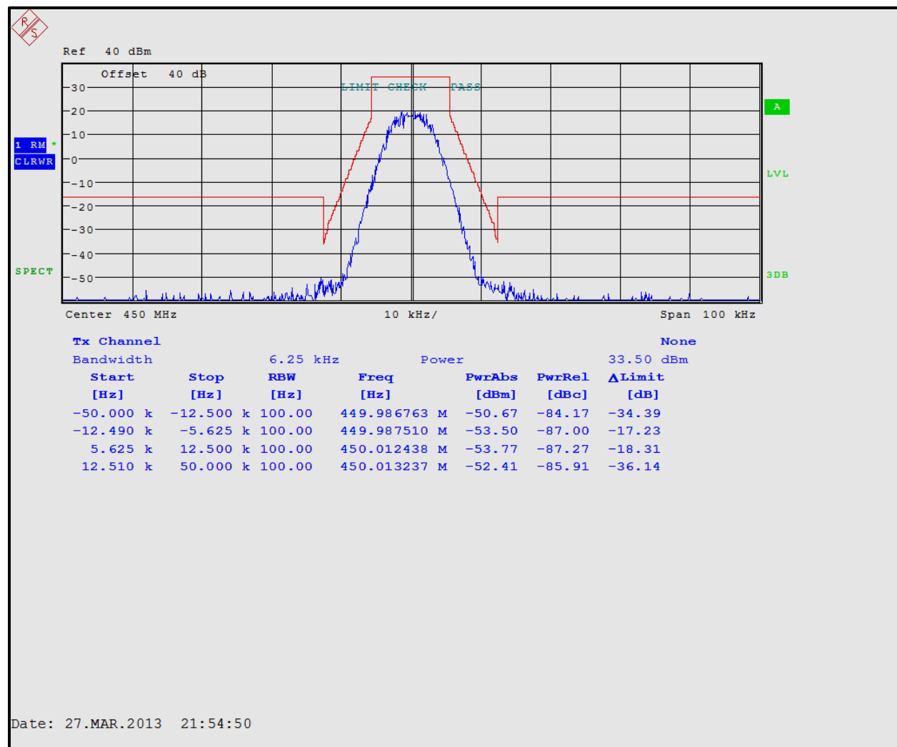
Plot 5-1: Occupied Bandwidth – 450 MHz; H-CPM TDMA (Mask D)
