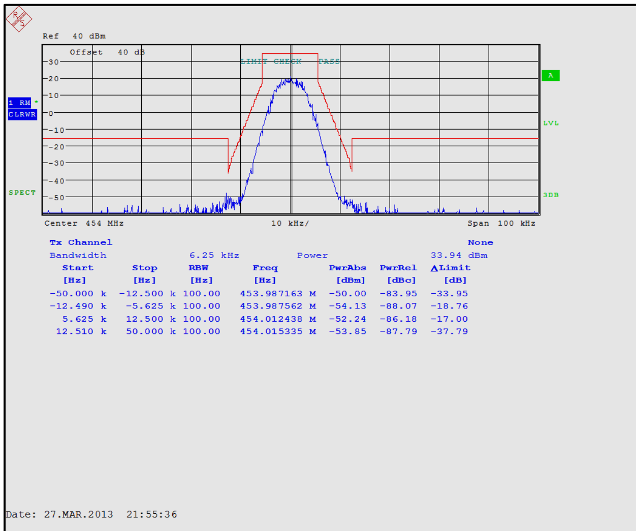
Plot 5-2: Occupied Bandwidth – 454.0000 MHz; H-CPM TDMA (Mask D)
