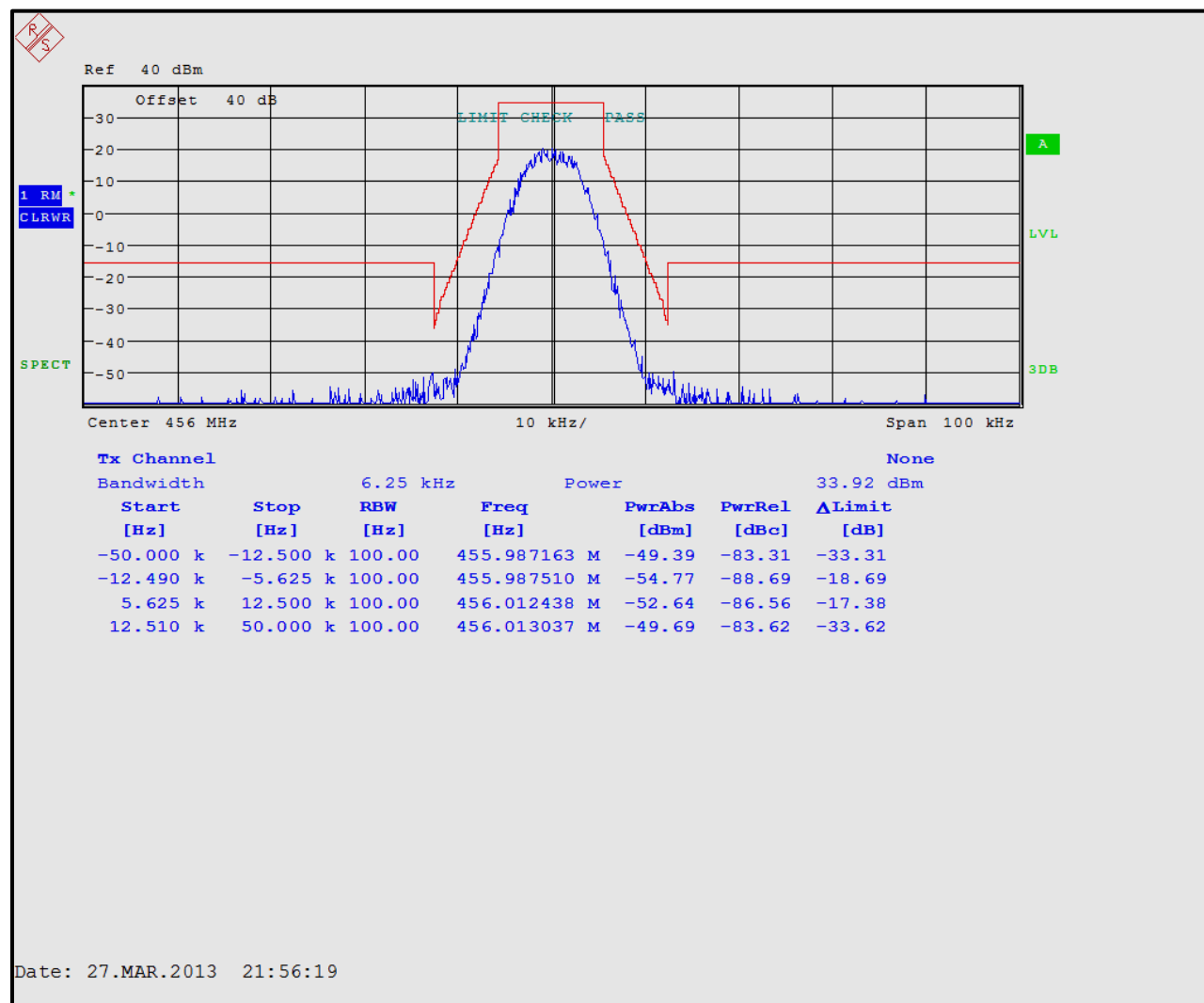
Plot 5-3: Occupied Bandwidth – 456.0000 MHz; H-CPM TDMA (Mask D)
