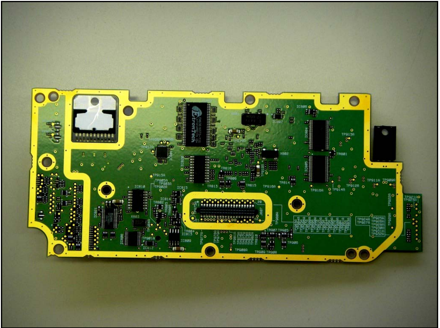
Photograph 8: PK Board – Solder Side
