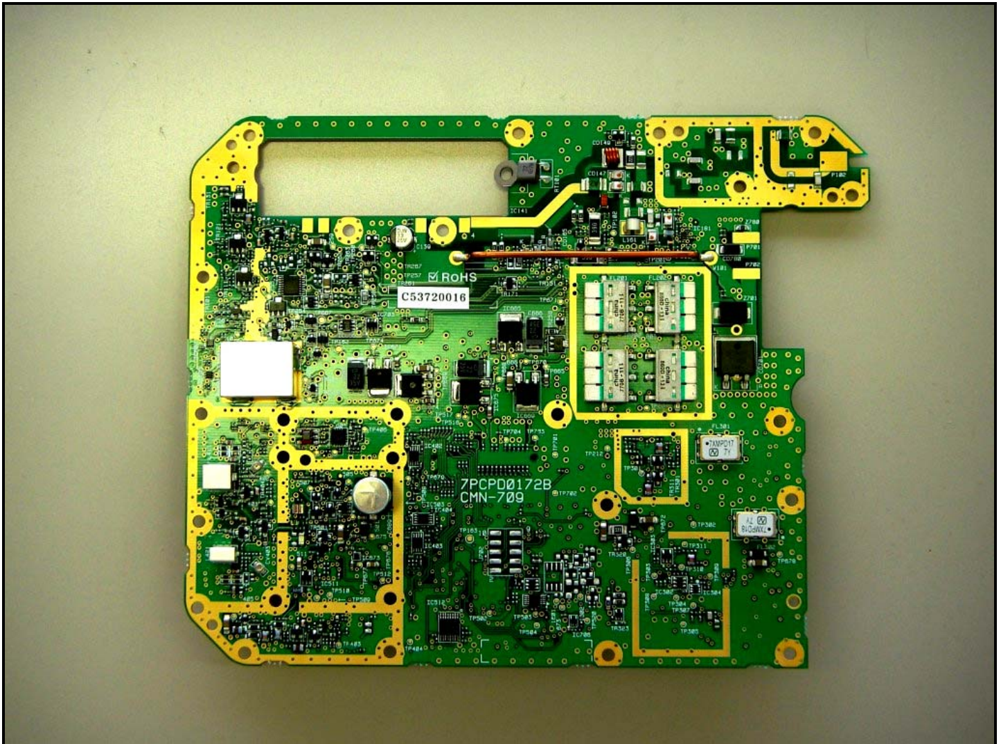
Photograph 5: RF Processor Board - Component Side
