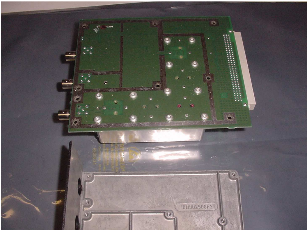
Figure 2 - Rx Front End Board Bottom View
