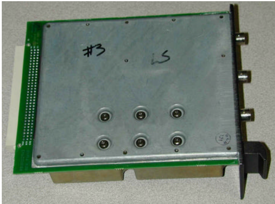
Figure 15: Low frequency split Rx Synthesizer Back View Cover On
