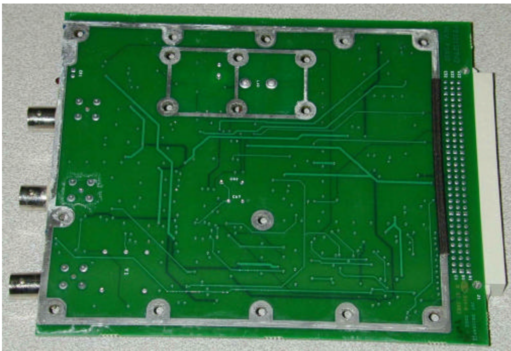
Figure 16: Low frequency split Rx Synthesizer Back View Cover Off
