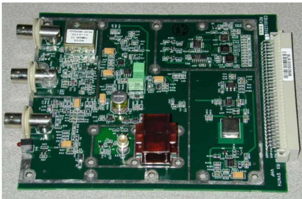
Figure 14: Low frequency split Rx Synthesizer Front View Cover Off
