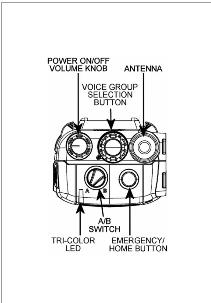
Figure 7-2: Top View
