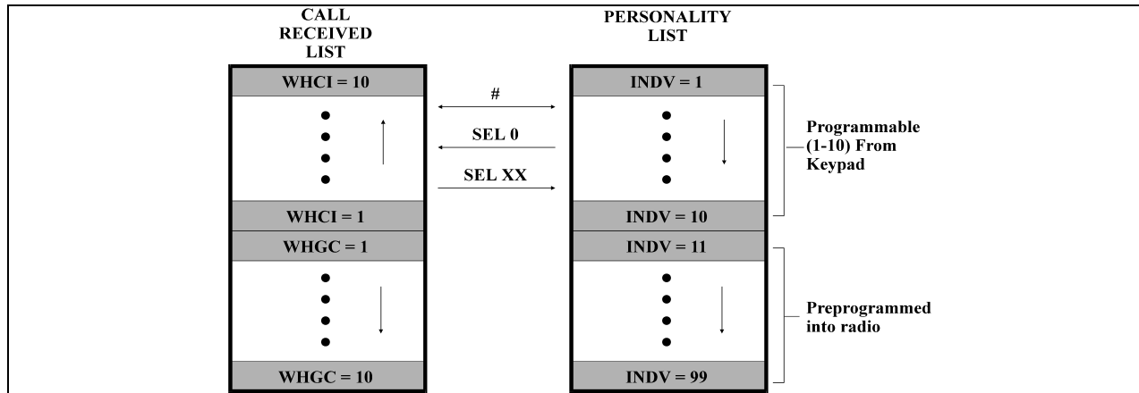
Figure 10-13: Calls Received and Personality Lists
