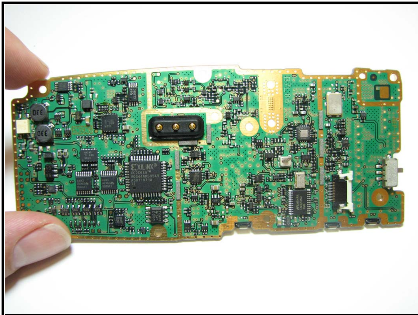
Photograph 18: Main Board - Bottom View
