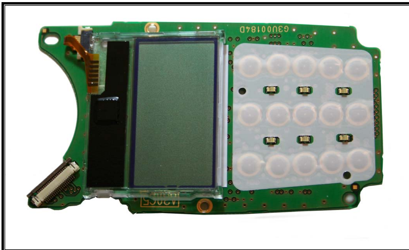
Photograph 20: Interface Board - Front View
