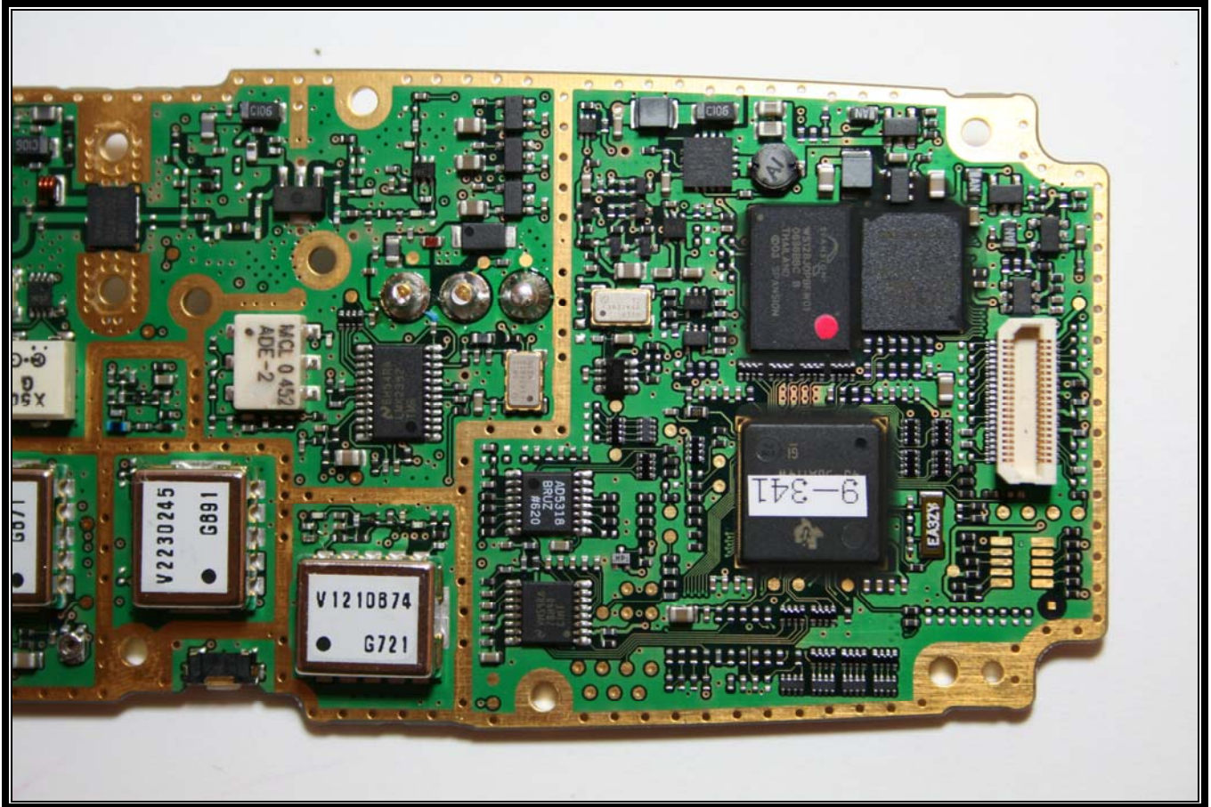
Photograph 17: Main Board – Top View Close Up of Logic Section
