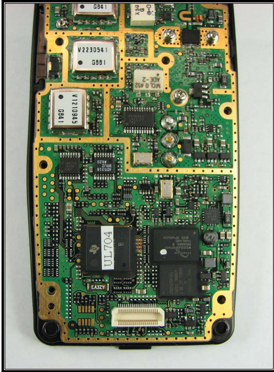
Photograph 11: Main Board in Casing – Top View 1
