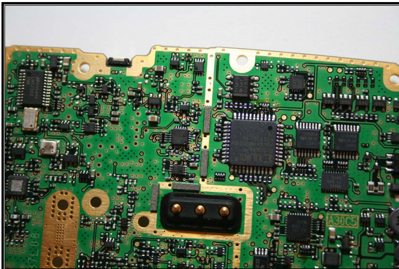
Photograph 19: Main Board - Bottom View Close Up of Battery Contact
