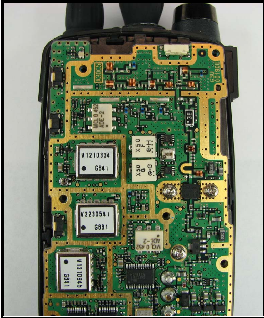
Photograph 12: Main Board in Casing - Top View 2
