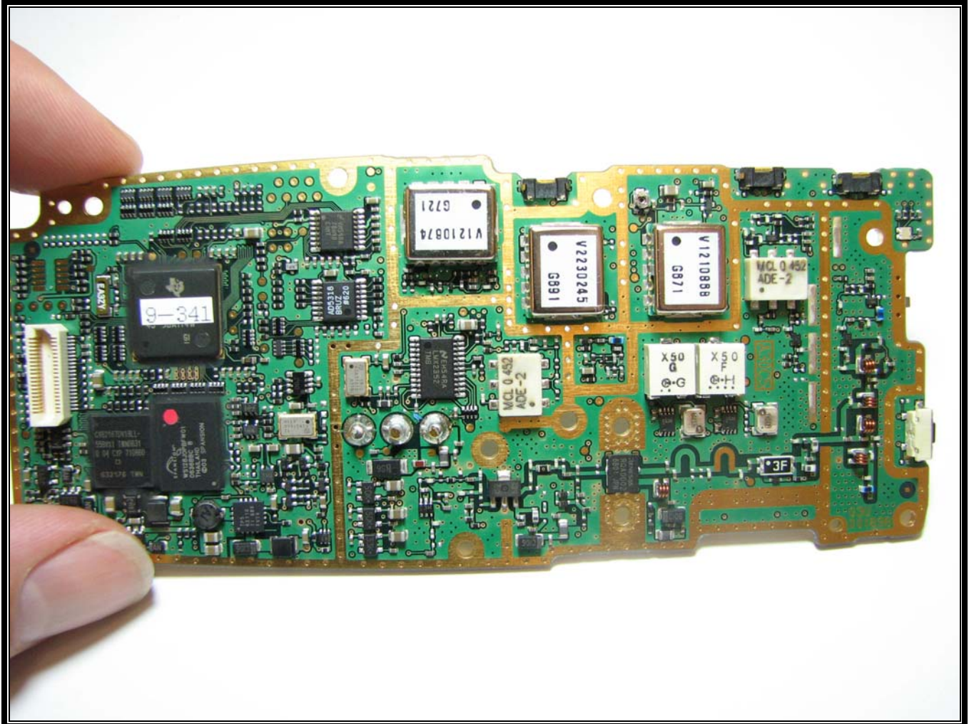
Photograph 16: Main Board - Top Overall View
