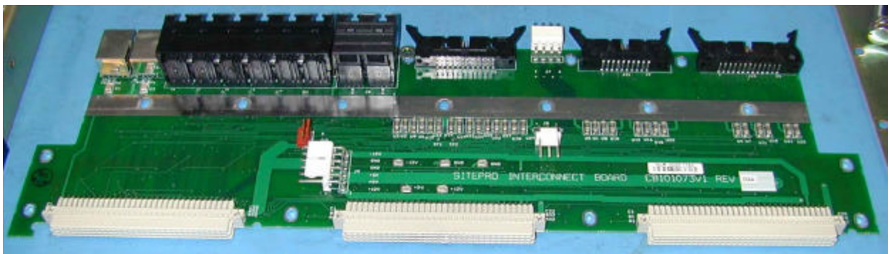
Figure 9: Stepro Interconnect Board, CB101073V1 Rev. R2A SLR 0228 1140, Top View
