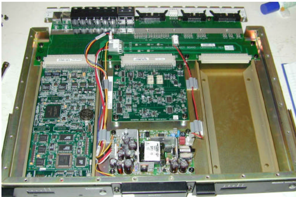
Figure 4: Top View of Module, No Cover
