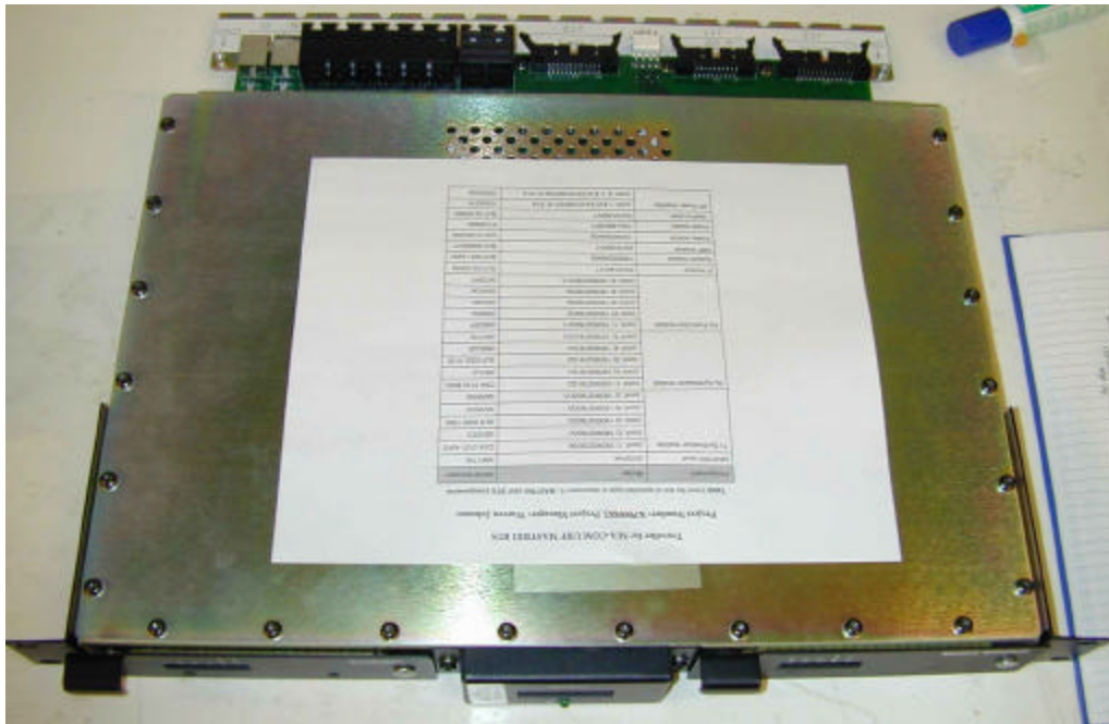
Figure 2: Front View of Module, Cover On
