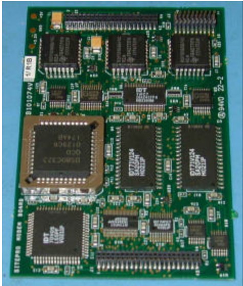
Figure 15: Daughterboard, SLR 0223 1249 T119 Jun 02,
