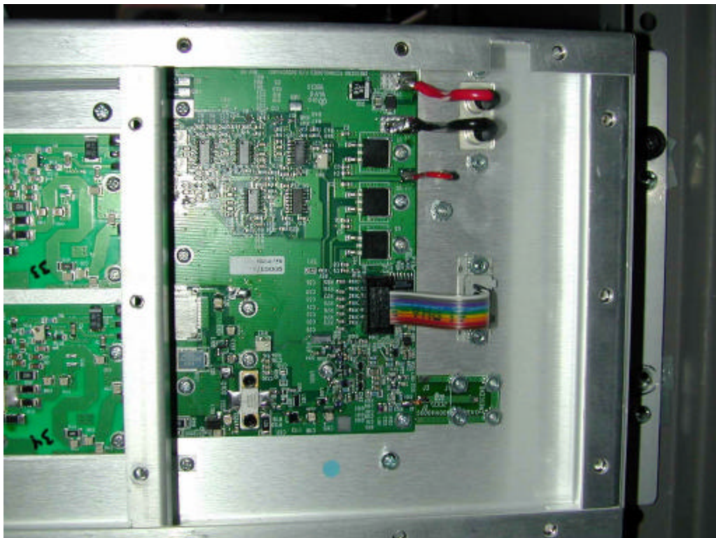
Figure 6: PA #1 Rightmost Section of Board
