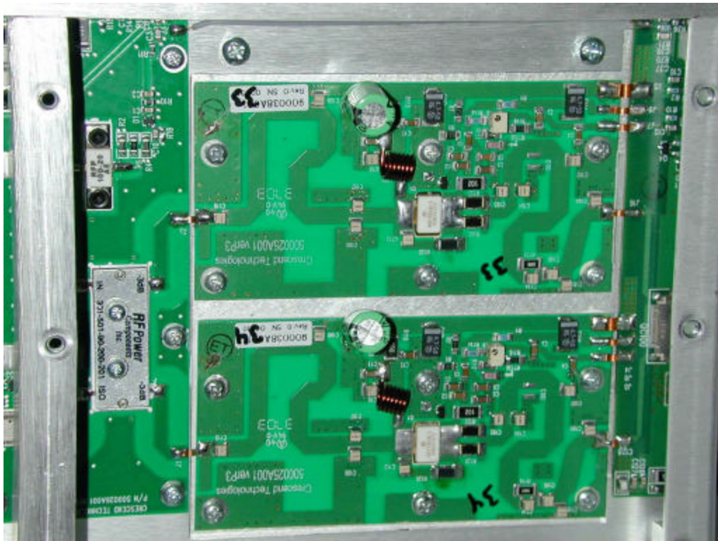
Figure 5: PA #1 Middle section of Board
