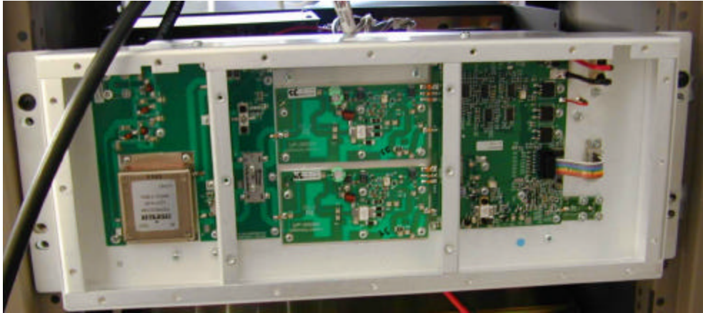
Figure 3: PA #1 SN 10325556 (Freq: 440-512 MHz)
