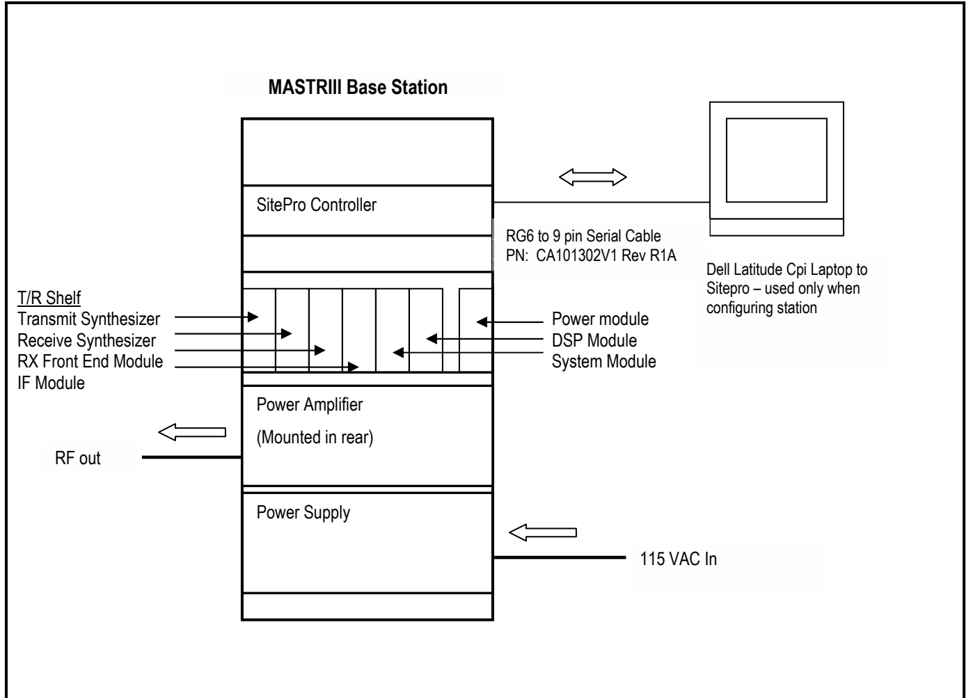
FIGURE 3-1: CONFIGURATION OF TESTED SYSTEM
