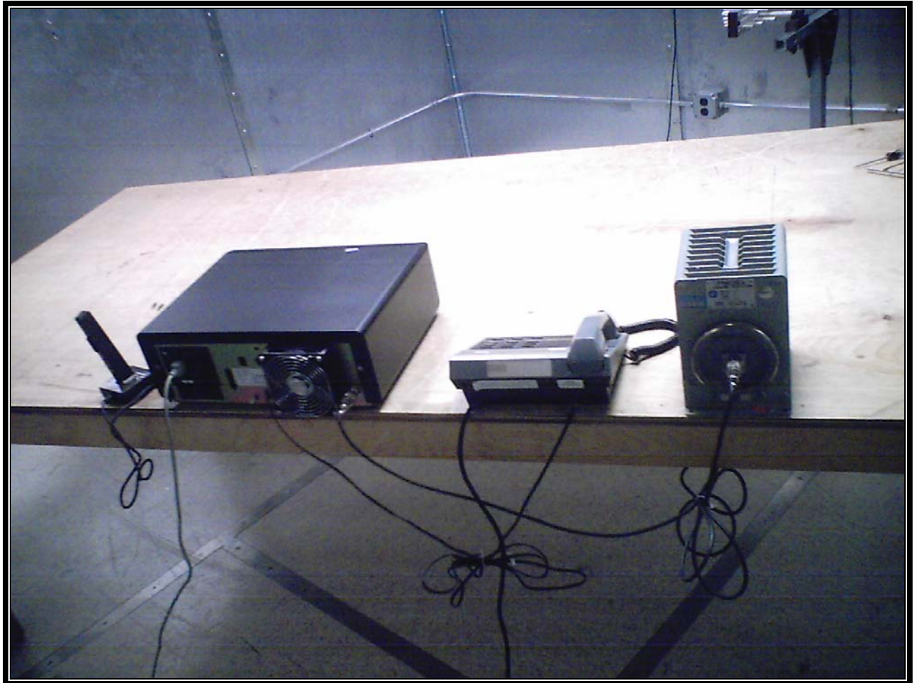
Photograph 8: Conducted Emissions (Rear View) Desktop Configuration
