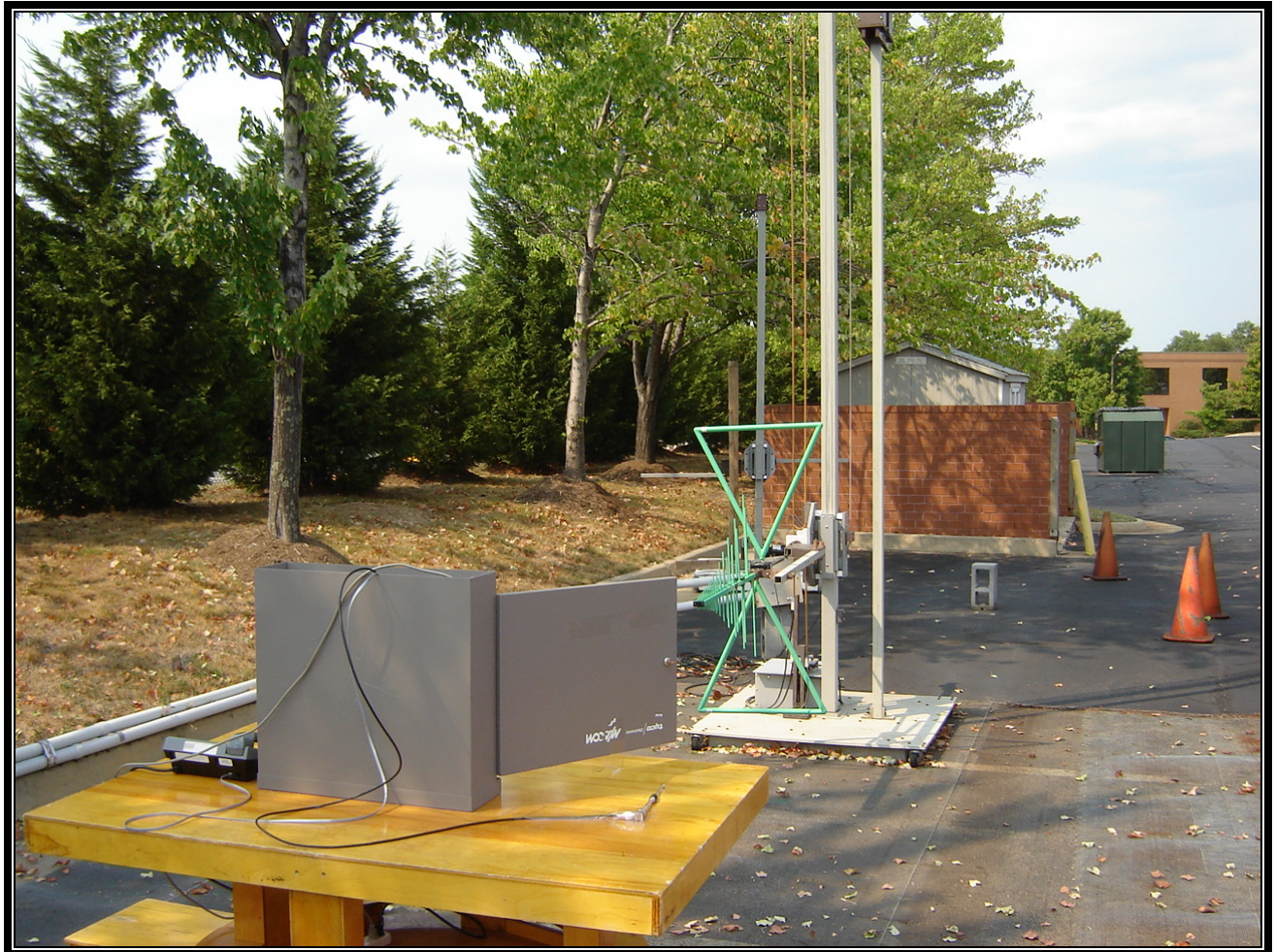
Photograph 2: Radiated Emissions (Rear View) Wall Mount Configuration
