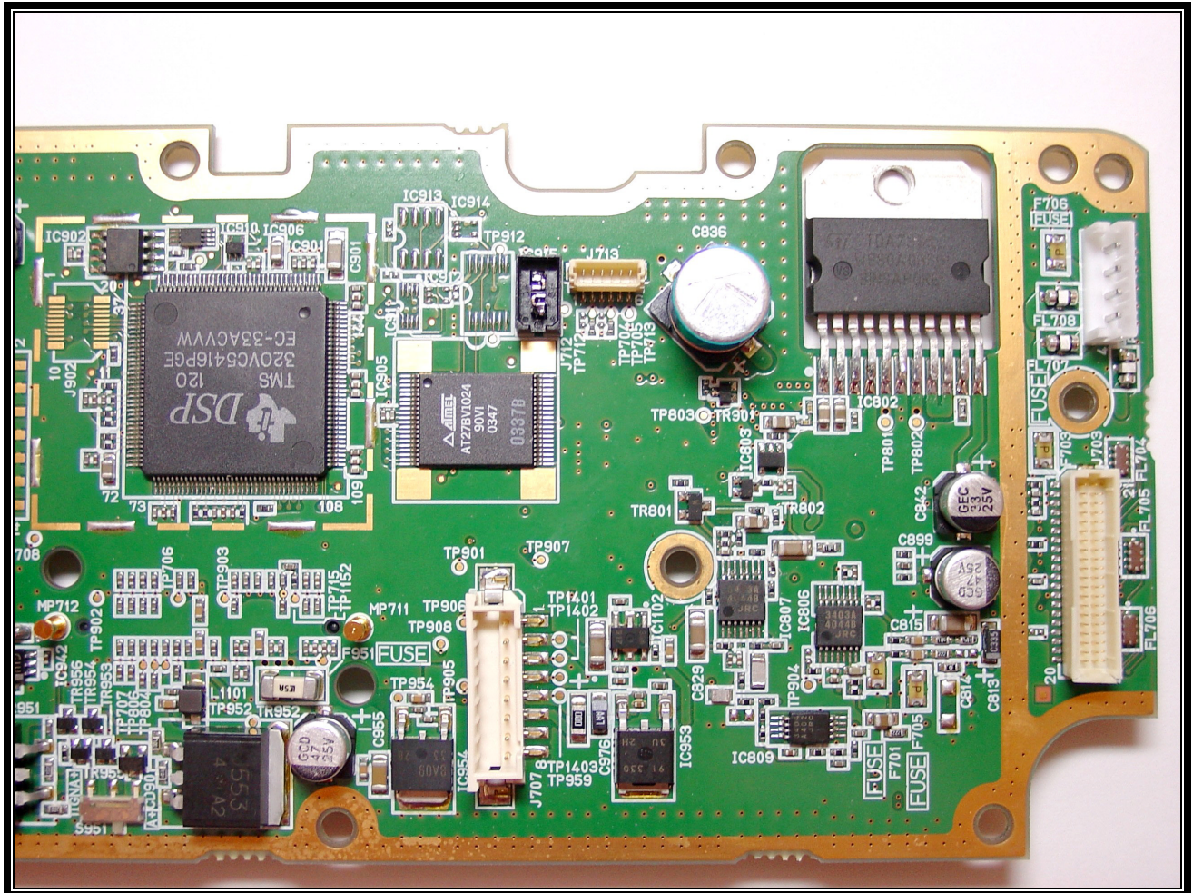
PHOTOGRAPH 8: AUDIO LOGIC BOARD COMPONENT SIDE – RIGHT
